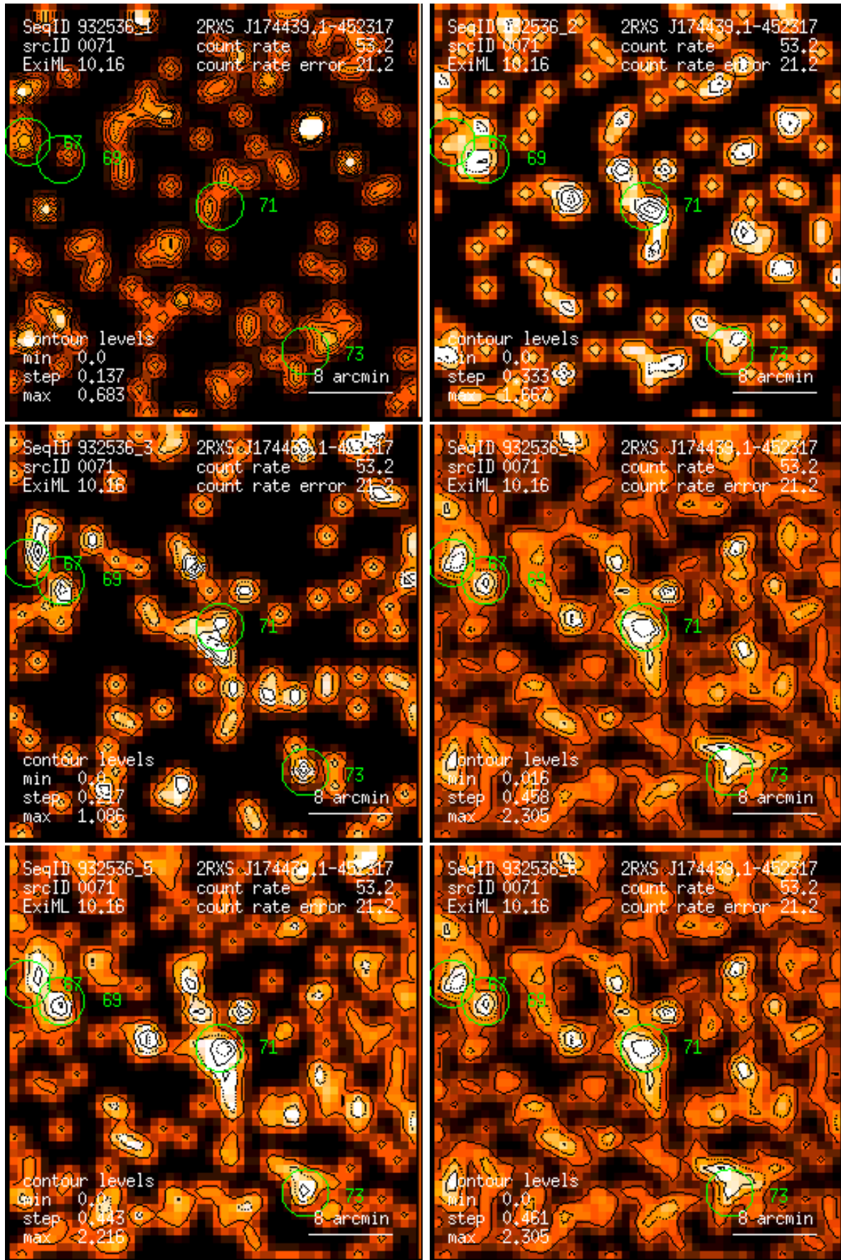
Figure 71: RASS 932536: detection 0071: band rate images, Gaussian filter: (1) PSPC channels 11 – 41, (2) 52 – 90, (3) 91 – 201, (4) 11 – 235, (5) 52 – 201, (6) 11 – 201. Broad band rates in counts/ks. Band rate contour levels in counts/ks/arcmin 2 .
