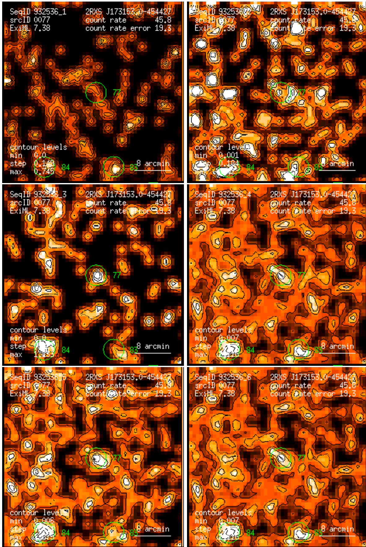
Figure 77: RASS 932536: detection 0077: band rate images, Gaussian filter: (1) PSPC channels 11 – 41, (2) 52 – 90, (3) 91 – 201, (4) 11 – 235, (5) 52 – 201, (6) 11 – 201. Broad band rates in counts/ks. Band rate contour levels in counts/ks/arcmin 2 .
