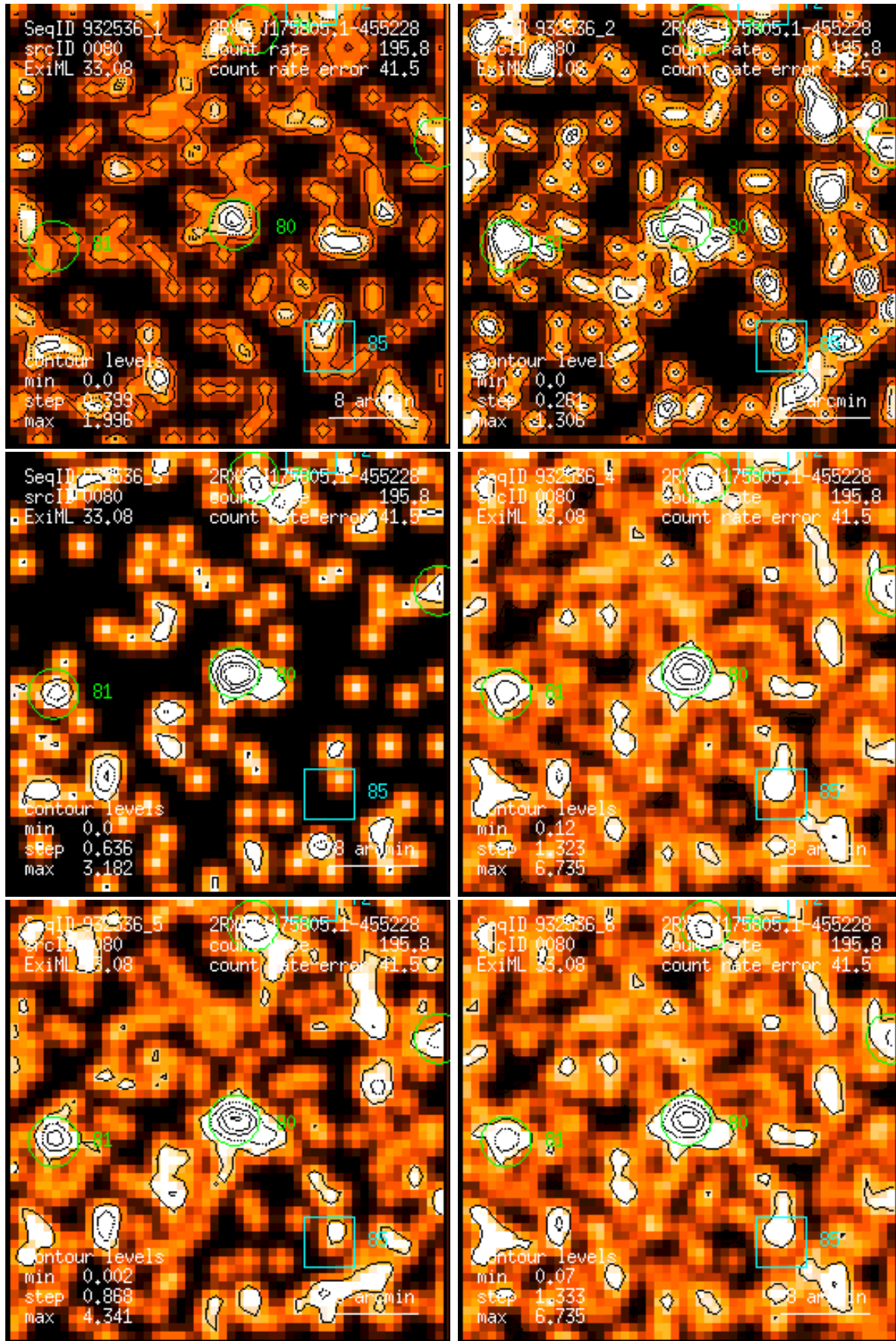
Figure 80: RASS 932536: detection 0080: band rate images, Gaussian filter: (1) PSPC channels 11 – 41, (2) 52 – 90, (3) 91 – 201, (4) 11 – 235, (5) 52 – 201, (6) 11 – 201. Broad band rates in counts/ks. Band rate contour levels in counts/ks/arcmin 2 .
