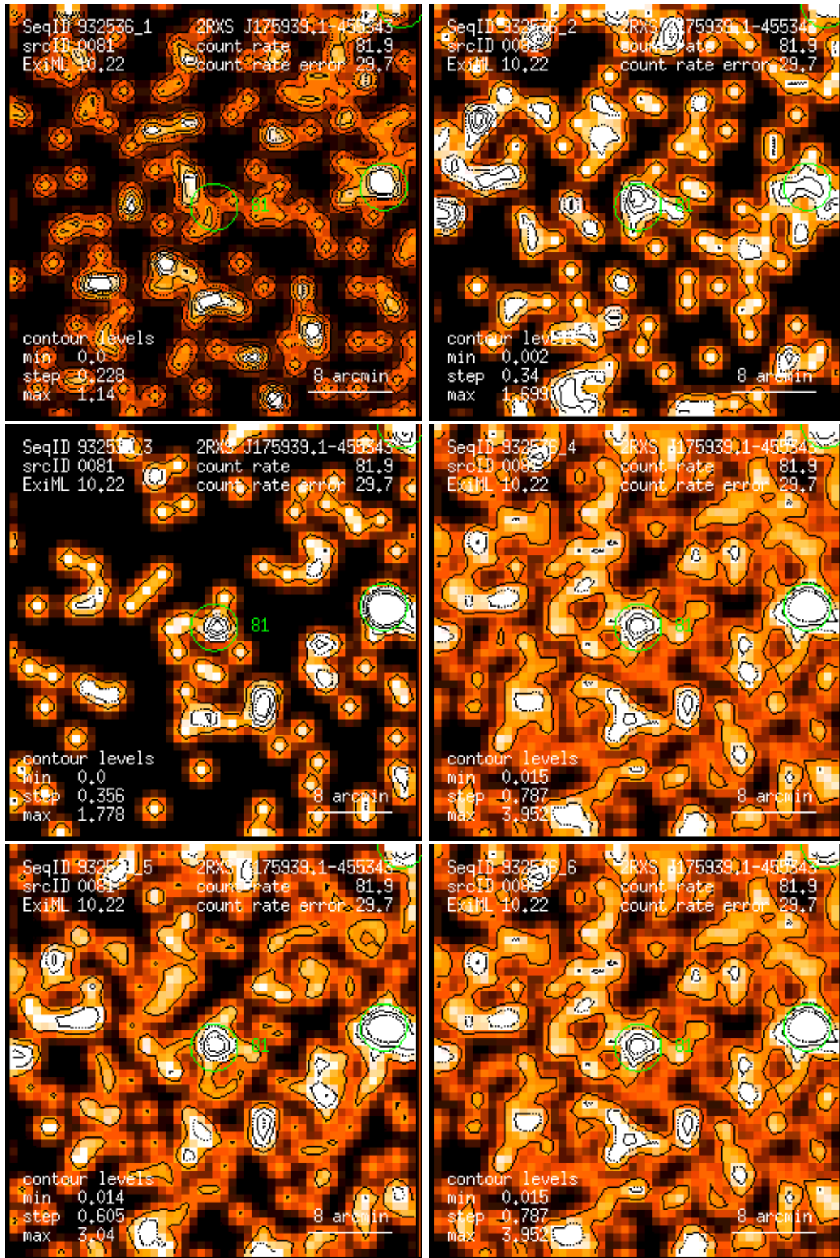
Figure 81: RASS 932536: detection 0081: band rate images, Gaussian filter: (1) PSPC channels 11 – 41, (2) 52 – 90, (3) 91 – 201, (4) 11 – 235, (5) 52 – 201, (6) 11 – 201. Broad band rates in counts/ks. Band rate contour levels in counts/ks/arcmin 2 .
