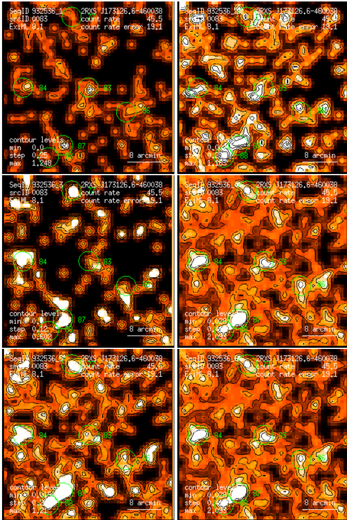
Figure 83: RASS 932536: detection 0083: band rate images, Gaussian filter: (1) PSPC channels 11 – 41, (2) 52 – 90, (3) 91 – 201, (4) 11 – 235, (5) 52 – 201, (6) 11 – 201. Broad band rates in counts/ks. Band rate contour levels in counts/ks/arcmin 2 .
