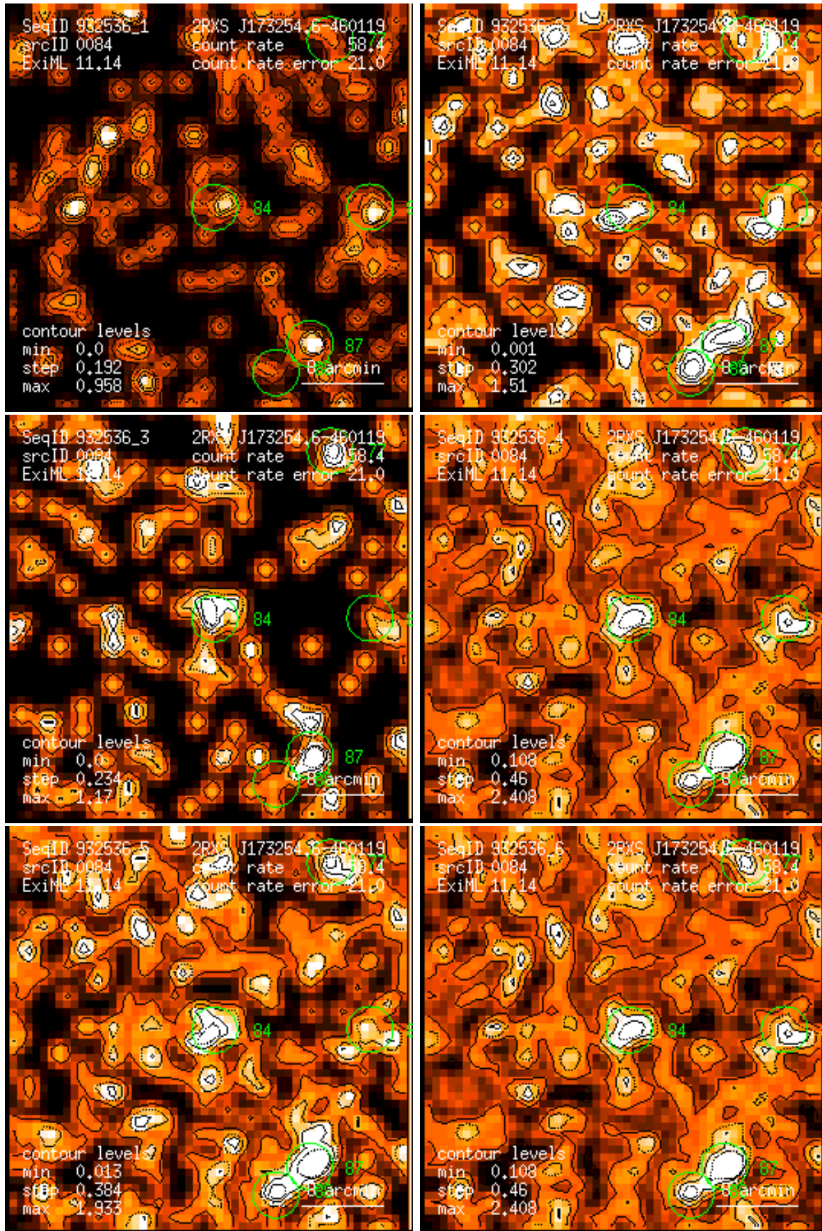
Figure 84: RASS 932536: detection 0084: band rate images, Gaussian filter: (1) PSPC channels 11 – 41, (2) 52 – 90, (3) 91 – 201, (4) 11 – 235, (5) 52 – 201, (6) 11 – 201. Broad band rates in counts/ks. Band rate contour levels in counts/ks/arcmin 2 .
