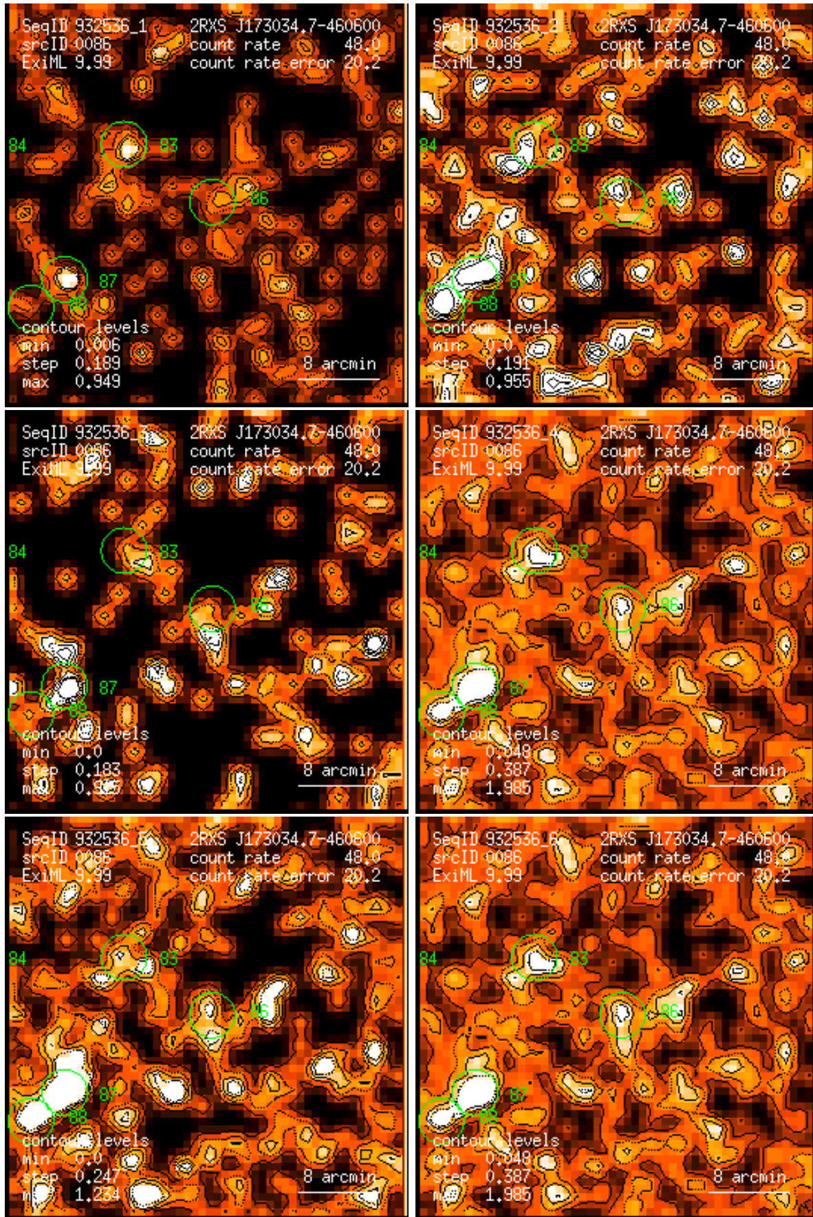
Figure 86: RASS 932536: detection 0086: band rate images, Gaussian filter: (1) PSPC channels 11 – 41, (2) 52 – 90, (3) 91 – 201, (4) 11 – 235, (5) 52 – 201, (6) 11 – 201. Broad band rates in counts/ks. Band rate contour levels in counts/ks/arcmin 2 .
