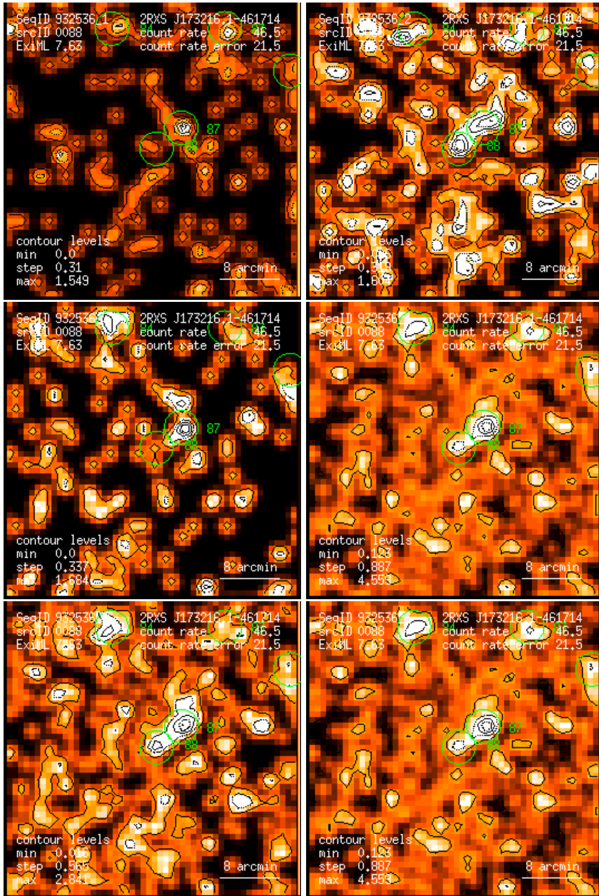
Figure 88: RASS 932536: detection 0088: band rate images, Gaussian filter: (1) PSPC channels 11 – 41, (2) 52 – 90, (3) 91 – 201, (4) 11 – 235, (5) 52 – 201, (6) 11 – 201. Broad band rates in counts/ks. Band rate contour levels in counts/ks/arcmin 2 .
