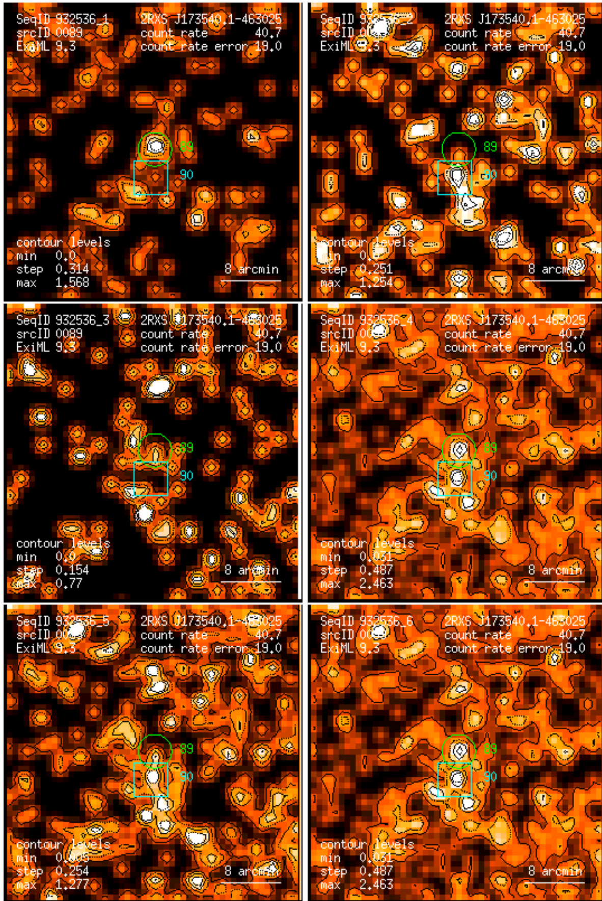
Figure 89: RASS 932536: detection 0089: band rate images, Gaussian filter: (1) PSPC channels 11 – 41, (2) 52 – 90, (3) 91 – 201, (4) 11 – 235, (5) 52 – 201, (6) 11 – 201. Broad band rates in counts/ks. Band rate contour levels in counts/ks/arcmin 2 .
