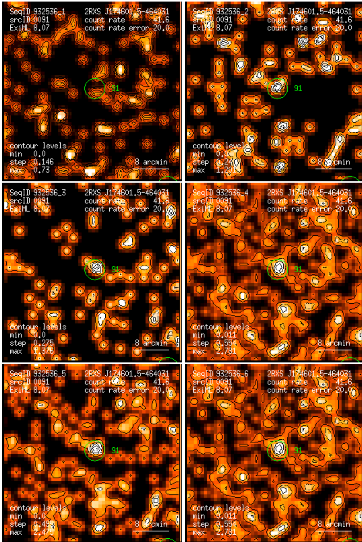
Figure 91: RASS 932536: detection 0091: band rate images, Gaussian filter: (1) PSPC channels 11 – 41, (2) 52 – 90, (3) 91 – 201, (4) 11 – 235, (5) 52 – 201, (6) 11 – 201. Broad band rates in counts/ks. Band rate contour levels in counts/ks/arcmin 2 .
