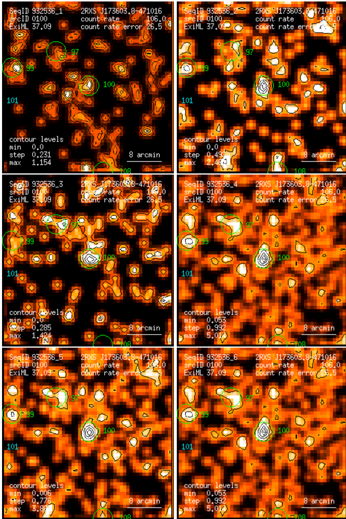
Figure 100: RASS 932536: detection 0100: band rate images, Gaussian filter: (1) PSPC channels 11 – 41, (2) 52 – 90, (3) 91 – 201, (4) 11 – 235, (5) 52 – 201, (6) 11 – 201. Broad band rates in counts/ks. Band rate contour levels in counts/ks/arcmin 2 .
