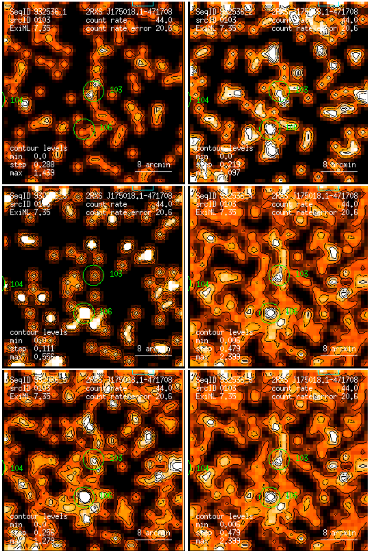
Figure 103: RASS 932536: detection 0103: band rate images, Gaussian filter: (1) PSPC channels 11 – 41, (2) 52 – 90, (3) 91 – 201, (4) 11 – 235, (5) 52 – 201, (6) 11 – 201. Broad band rates in counts/ks. Band rate contour levels in counts/ks/arcmin 2 .
