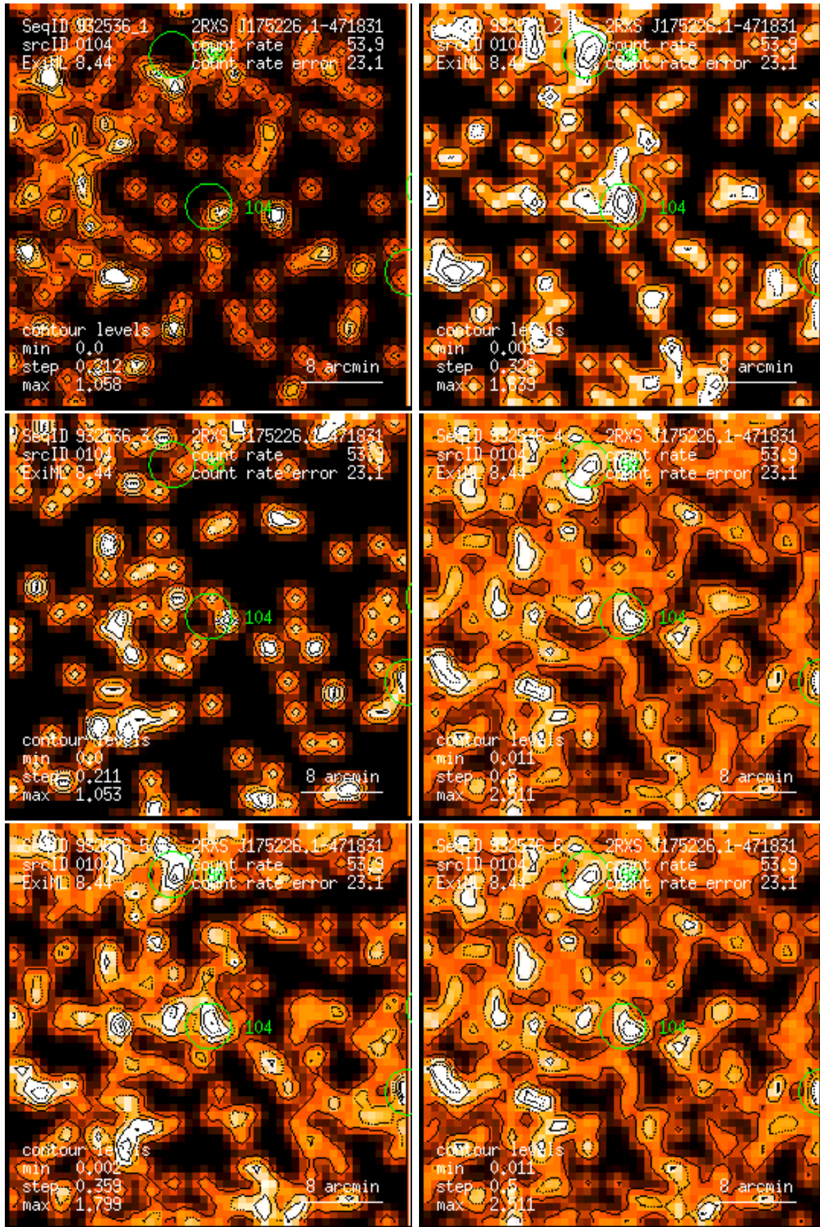
Figure 104: RASS 932536: detection 0104: band rate images, Gaussian filter: (1) PSPC channels 11 – 41, (2) 52 – 90, (3) 91 – 201, (4) 11 – 235, (5) 52 – 201, (6) 11 – 201. Broad band rates in counts/ks. Band rate contour levels in counts/ks/arcmin 2 .
