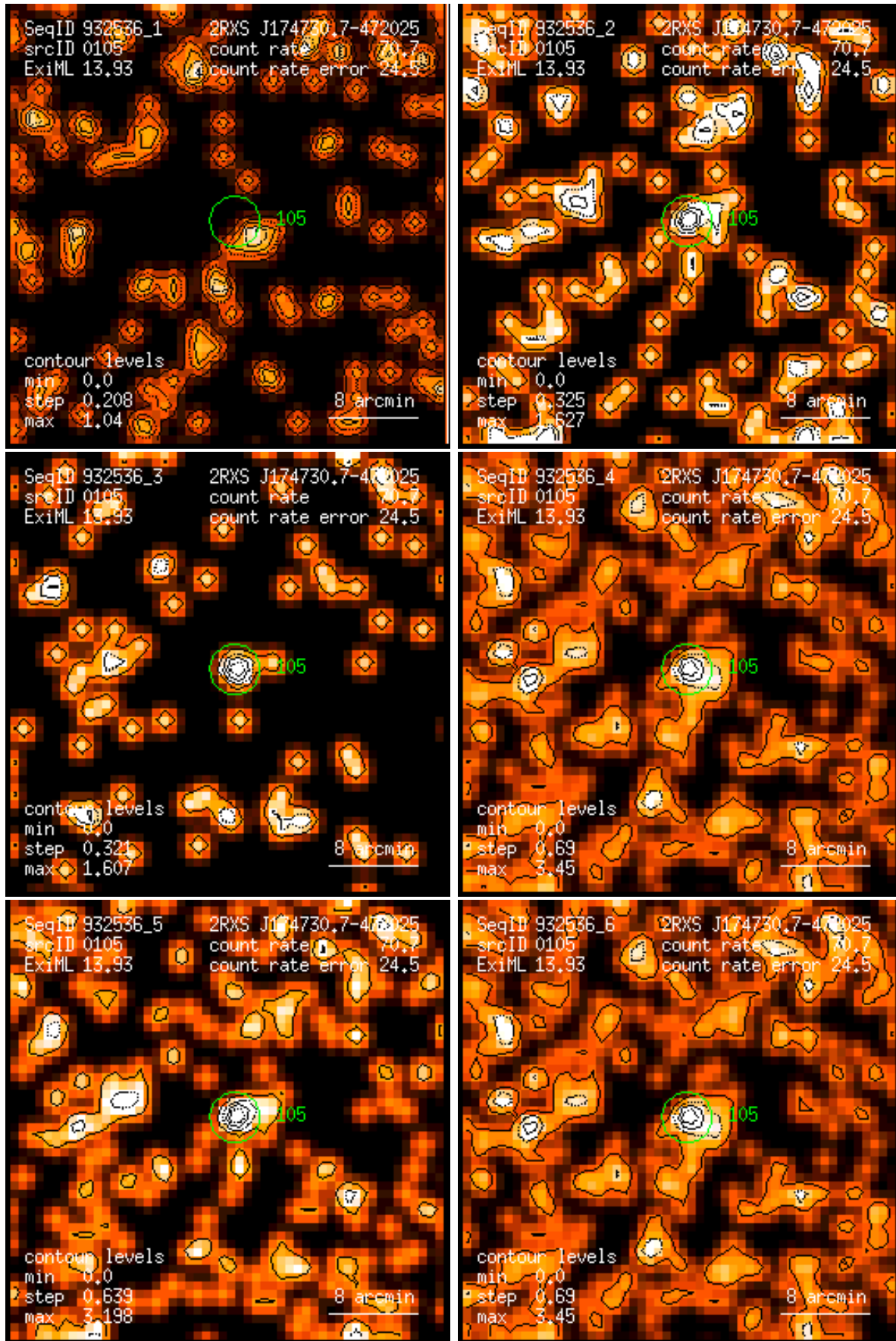
Figure 105: RASS 932536: detection 0105: band rate images, Gaussian filter: (1) PSPC channels 11 – 41, (2) 52 – 90, (3) 91 – 201, (4) 11 – 235, (5) 52 – 201, (6) 11 – 201. Broad band rates in counts/ks. Band rate contour levels in counts/ks/arcmin 2 .
