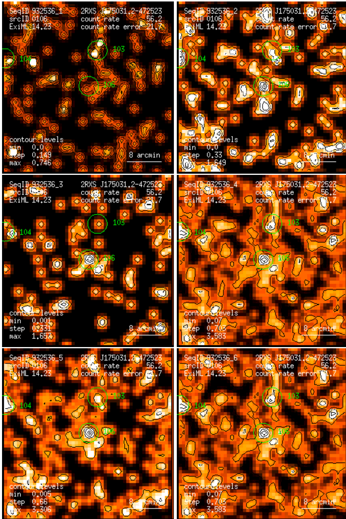
Figure 106: RASS 932536: detection 0106: band rate images, Gaussian filter: (1) PSPC channels 11 – 41, (2) 52 – 90, (3) 91 – 201, (4) 11 – 235, (5) 52 – 201, (6) 11 – 201. Broad band rates in counts/ks. Band rate contour levels in counts/ks/arcmin 2 .
