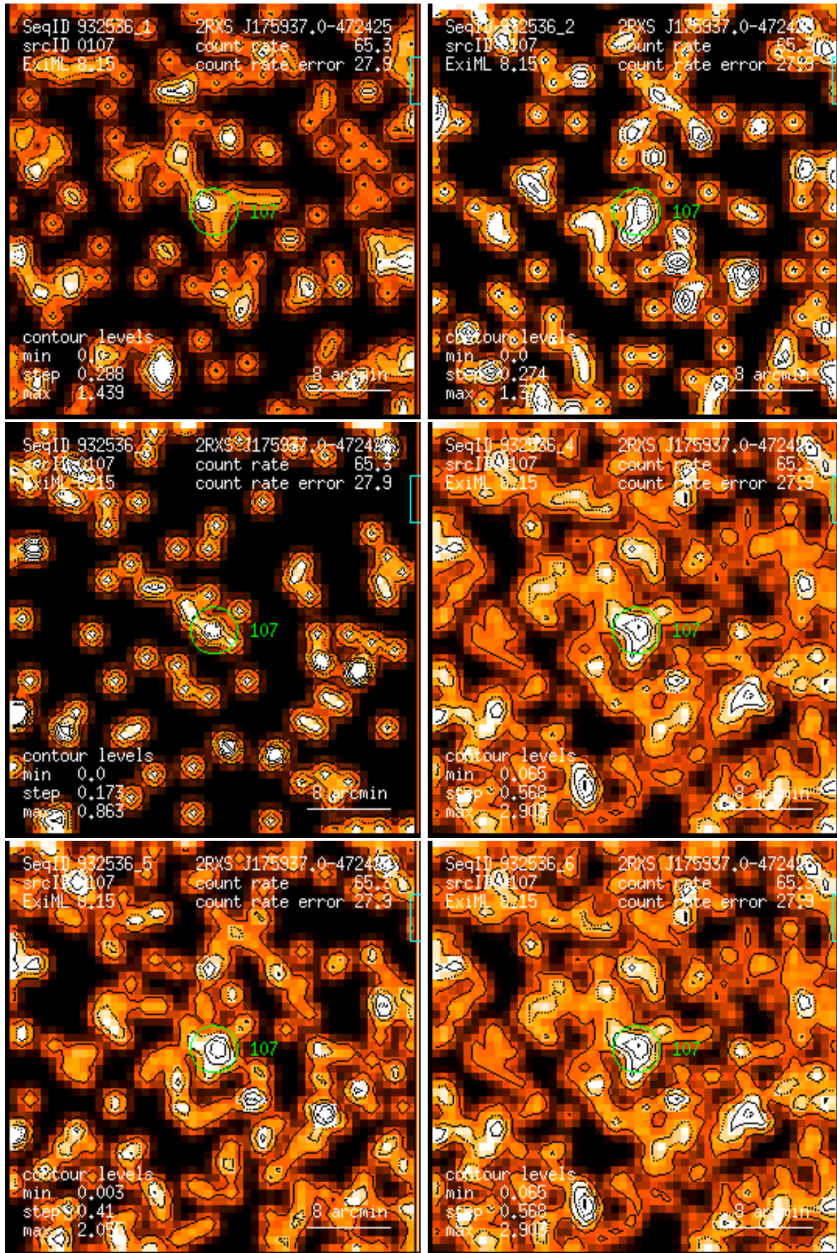
Figure 107: RASS 932536: detection 0107: band rate images, Gaussian filter: (1) PSPC channels 11 – 41, (2) 52 – 90, (3) 91 – 201, (4) 11 – 235, (5) 52 – 201, (6) 11 – 201. Broad band rates in counts/ks. Band rate contour levels in counts/ks/arcmin 2 .
