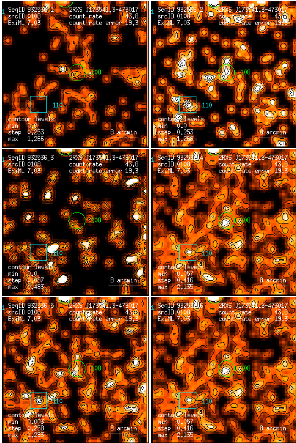
Figure 108: RASS 932536: detection 0108: band rate images, Gaussian filter: (1) PSPC channels 11 – 41, (2) 52 – 90, (3) 91 – 201, (4) 11 – 235, (5) 52 – 201, (6) 11 – 201. Broad band rates in counts/ks. Band rate contour levels in counts/ks/arcmin 2 .
