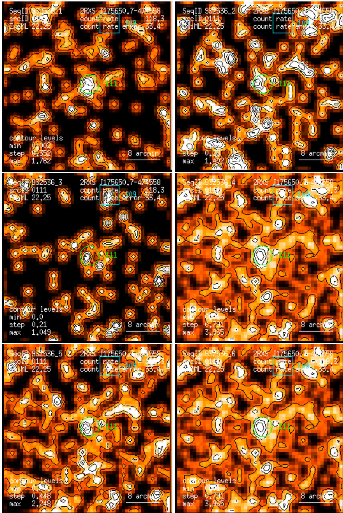
Figure 111: RASS 932536: detection 0111: band rate images, Gaussian filter: (1) PSPC channels 11 – 41, (2) 52 – 90, (3) 91 – 201, (4) 11 – 235, (5) 52 – 201, (6) 11 – 201. Broad band rates in counts/ks. Band rate contour levels in counts/ks/arcmin 2 .
