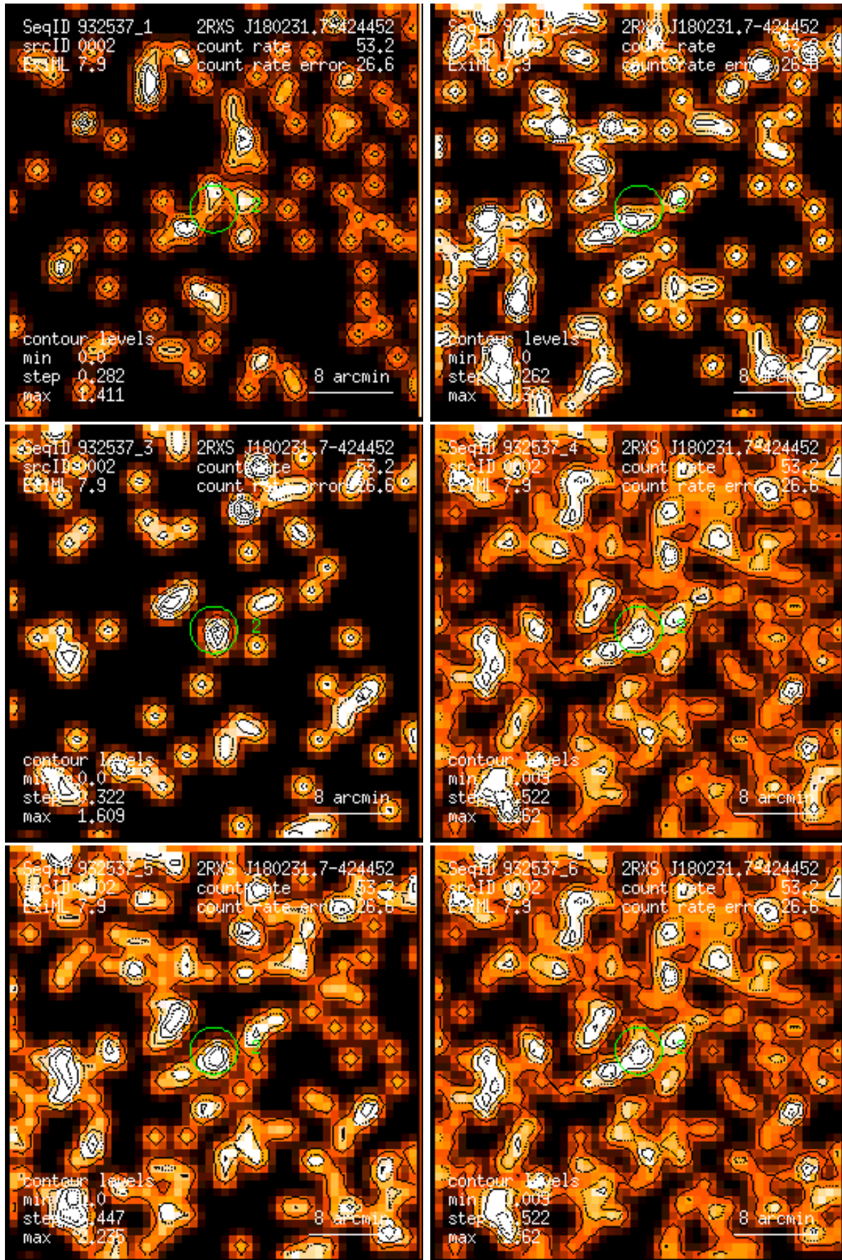
Figure 2: RASS 932537: detection 0002: band rate images, Gaussian filter: (1) PSPC channels 11 – 41, (2) 52 – 90, (3) 91 – 201, (4) 11 – 235, (5) 52 – 201, (6) 11 – 201. Broad band rates in counts/ks. Band rate contour levels in counts/ks/arcmin 2 .
