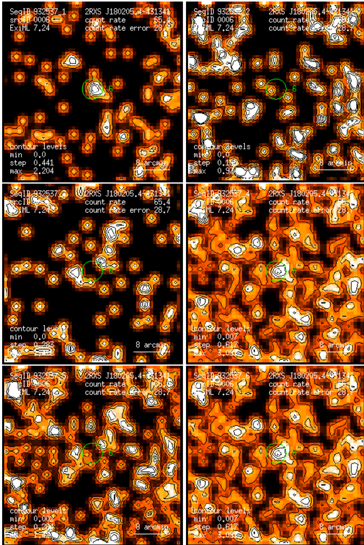
Figure 6: RASS 932537: detection 0006: band rate images, Gaussian filter: (1) PSPC channels 11 – 41, (2) 52 – 90, (3) 91 – 201, (4) 11 – 235, (5) 52 – 201, (6) 11 – 201. Broad band rates in counts/ks. Band rate contour levels in counts/ks/arcmin 2 .
