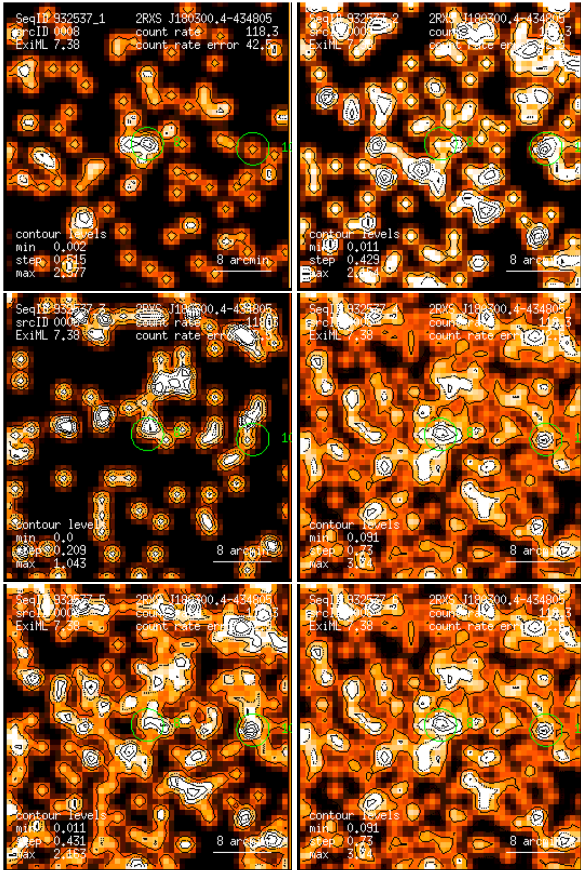
Figure 8: RASS 932537: detection 0008: band rate images, Gaussian filter: (1) PSPC channels 11 – 41, (2) 52 – 90, (3) 91 – 201, (4) 11 – 235, (5) 52 – 201, (6) 11 – 201. Broad band rates in counts/ks. Band rate contour levels in counts/ks/arcmin 2 .
