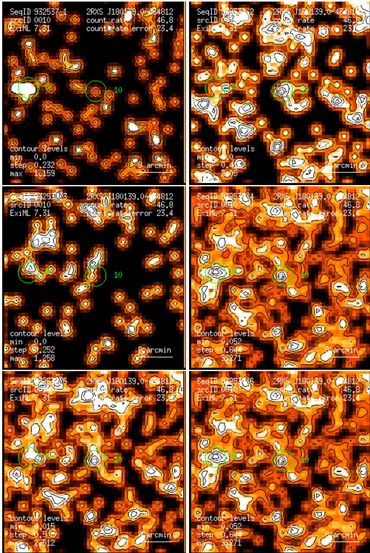
Figure 10: RASS 932537: detection 0010: band rate images, Gaussian filter: (1) PSPC channels 11 – 41, (2) 52 – 90, (3) 91 – 201, (4) 11 – 235, (5) 52 – 201, (6) 11 – 201. Broad band rates in counts/ks. Band rate contour levels in counts/ks/arcmin 2 .
