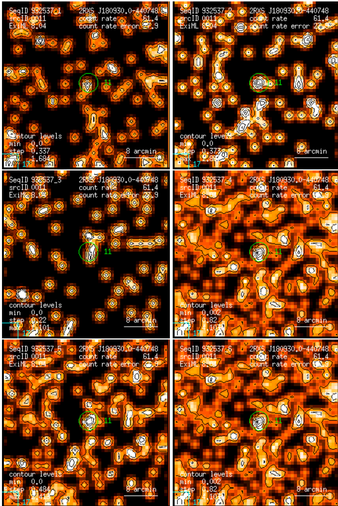
Figure 11: RASS 932537: detection 0011: band rate images, Gaussian filter: (1) PSPC channels 11 – 41, (2) 52 – 90, (3) 91 – 201, (4) 11 – 235, (5) 52 – 201, (6) 11 – 201. Broad band rates in counts/ks. Band rate contour levels in counts/ks/arcmin 2 .
