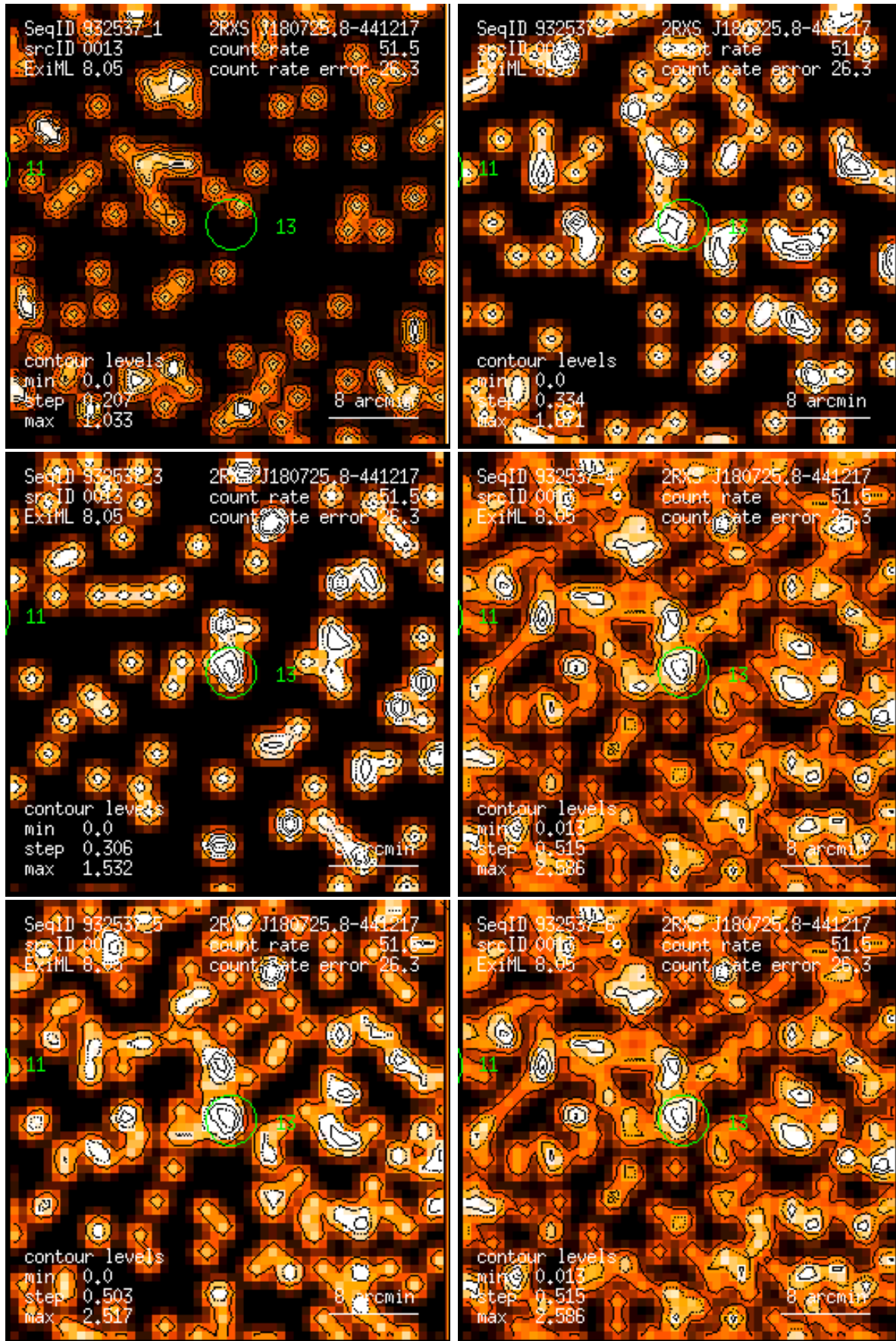
Figure 13: RASS 932537: detection 0013: band rate images, Gaussian filter: (1) PSPC channels 11 – 41, (2) 52 – 90, (3) 91 – 201, (4) 11 – 235, (5) 52 – 201, (6) 11 – 201. Broad band rates in counts/ks. Band rate contour levels in counts/ks/arcmin 2 .
