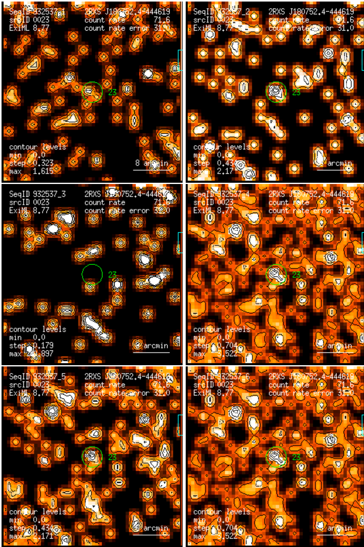
Figure 23: RASS 932537: detection 0023: band rate images, Gaussian filter: (1) PSPC channels 11 – 41, (2) 52 – 90, (3) 91 – 201, (4) 11 – 235, (5) 52 – 201, (6) 11 – 201. Broad band rates in counts/ks. Band rate contour levels in counts/ks/arcmin 2 .
