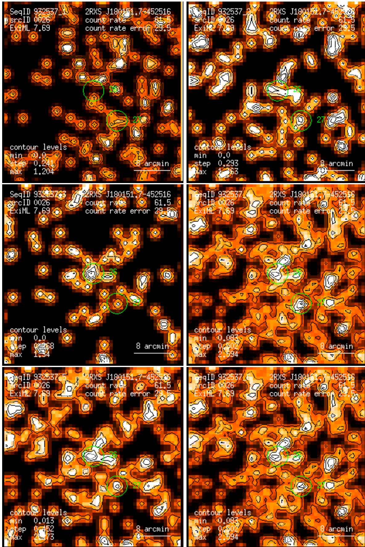
Figure 26: RASS 932537: detection 0026: band rate images, Gaussian filter: (1) PSPC channels 11 – 41, (2) 52 – 90, (3) 91 – 201, (4) 11 – 235, (5) 52 – 201, (6) 11 – 201. Broad band rates in counts/ks. Band rate contour levels in counts/ks/arcmin 2 .
