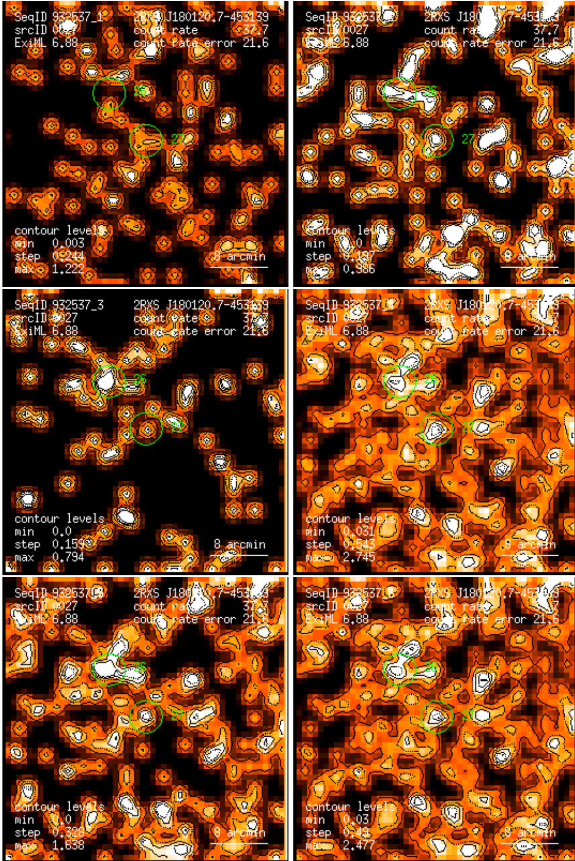
Figure 27: RASS 932537: detection 0027: band rate images, Gaussian filter: (1) PSPC channels 11 – 41, (2) 52 – 90, (3) 91 – 201, (4) 11 – 235, (5) 52 – 201, (6) 11 – 201. Broad band rates in counts/ks. Band rate contour levels in counts/ks/arcmin 2 .
