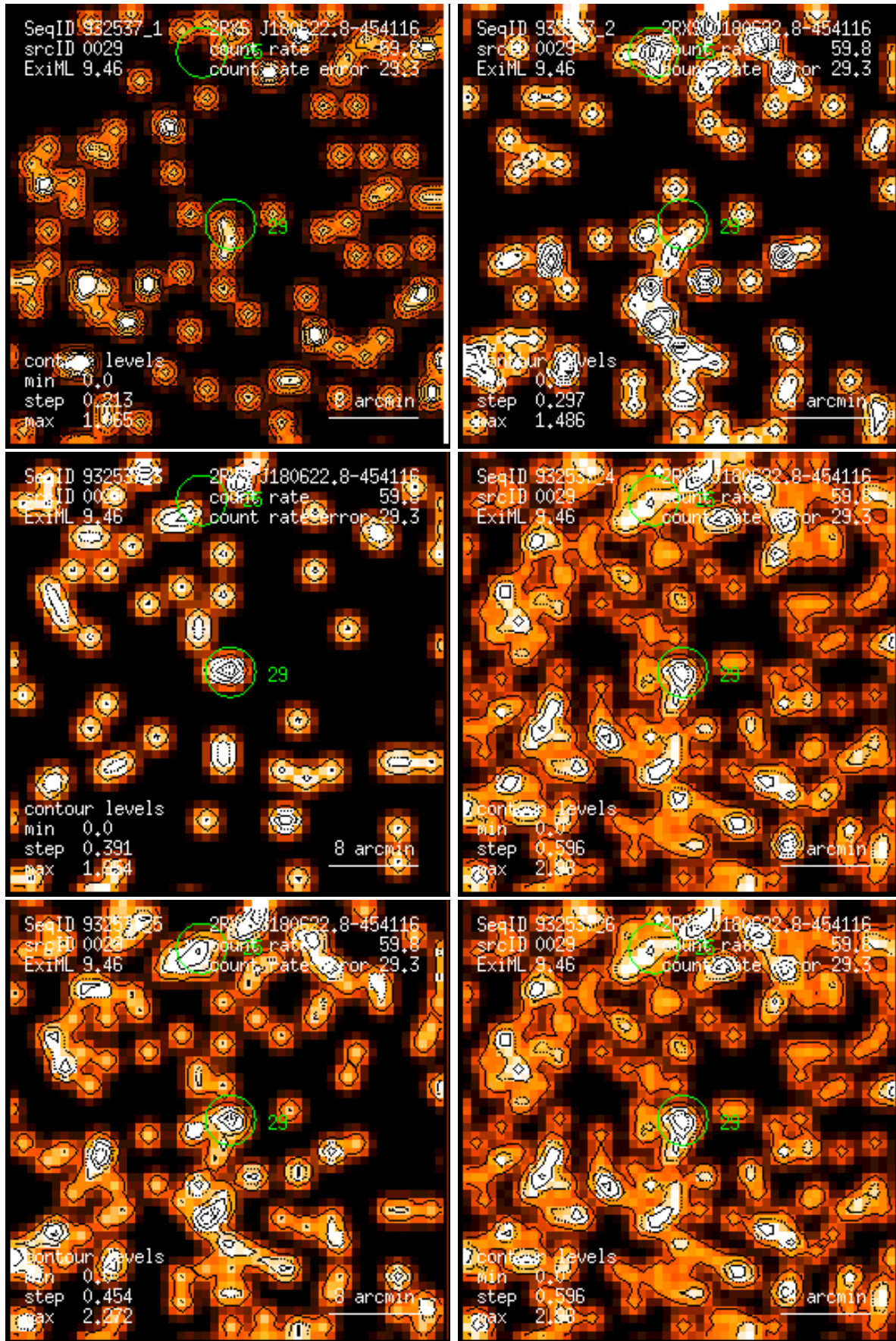
Figure 29: RASS 932537: detection 0029: band rate images, Gaussian filter: (1) PSPC channels 11 – 41, (2) 52 – 90, (3) 91 – 201, (4) 11 – 235, (5) 52 – 201, (6) 11 – 201. Broad band rates in counts/ks. Band rate contour levels in counts/ks/arcmin 2 .
