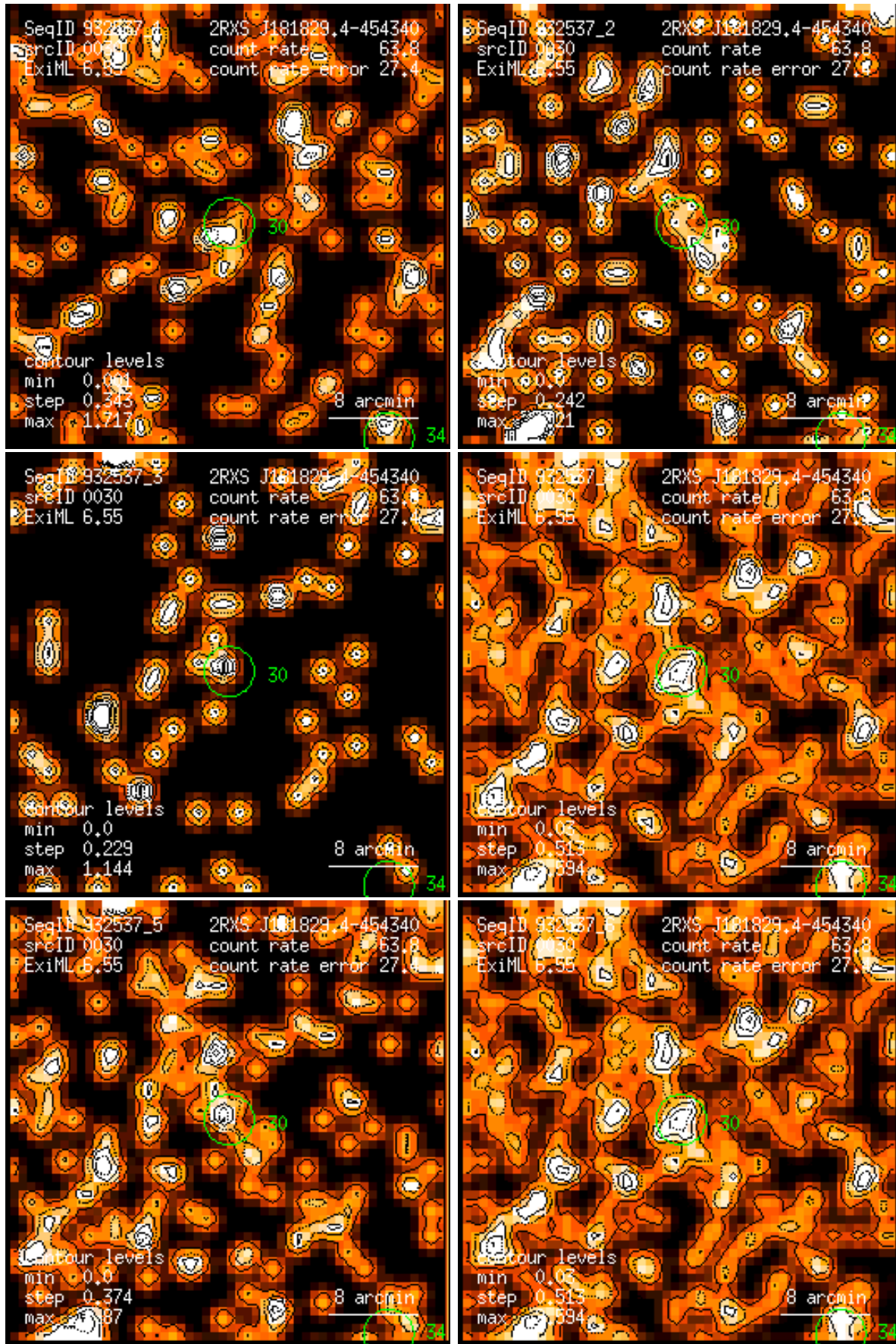
Figure 30: RASS 932537: detection 0030: band rate images, Gaussian filter: (1) PSPC channels 11 – 41, (2) 52 – 90, (3) 91 – 201, (4) 11 – 235, (5) 52 – 201, (6) 11 – 201. Broad band rates in counts/ks. Band rate contour levels in counts/ks/arcmin 2 .
