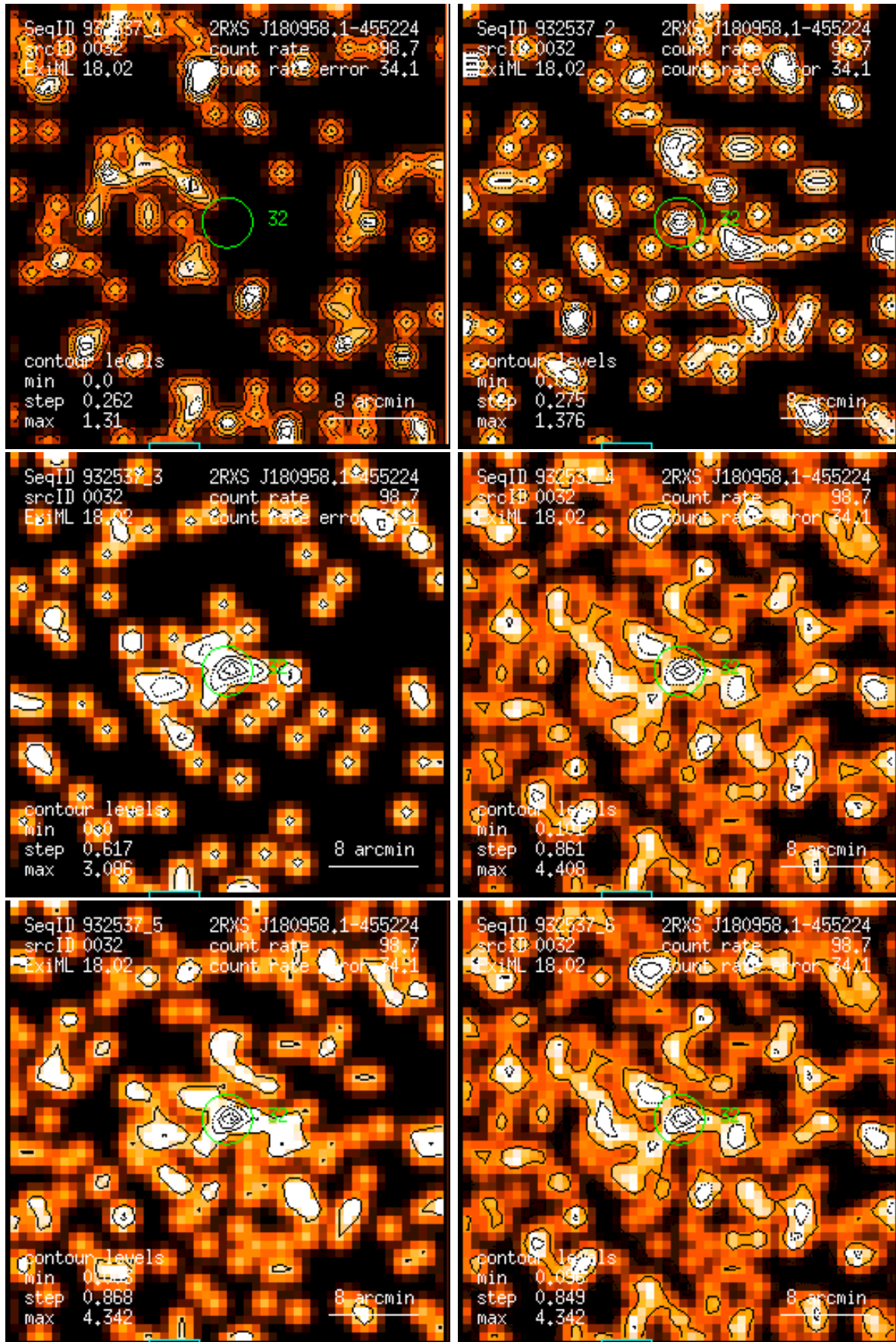
Figure 32: RASS 932537: detection 0032: band rate images, Gaussian filter: (1) PSPC channels 11 – 41, (2) 52 – 90, (3) 91 – 201, (4) 11 – 235, (5) 52 – 201, (6) 11 – 201. Broad band rates in counts/ks. Band rate contour levels in counts/ks/arcmin 2 .
