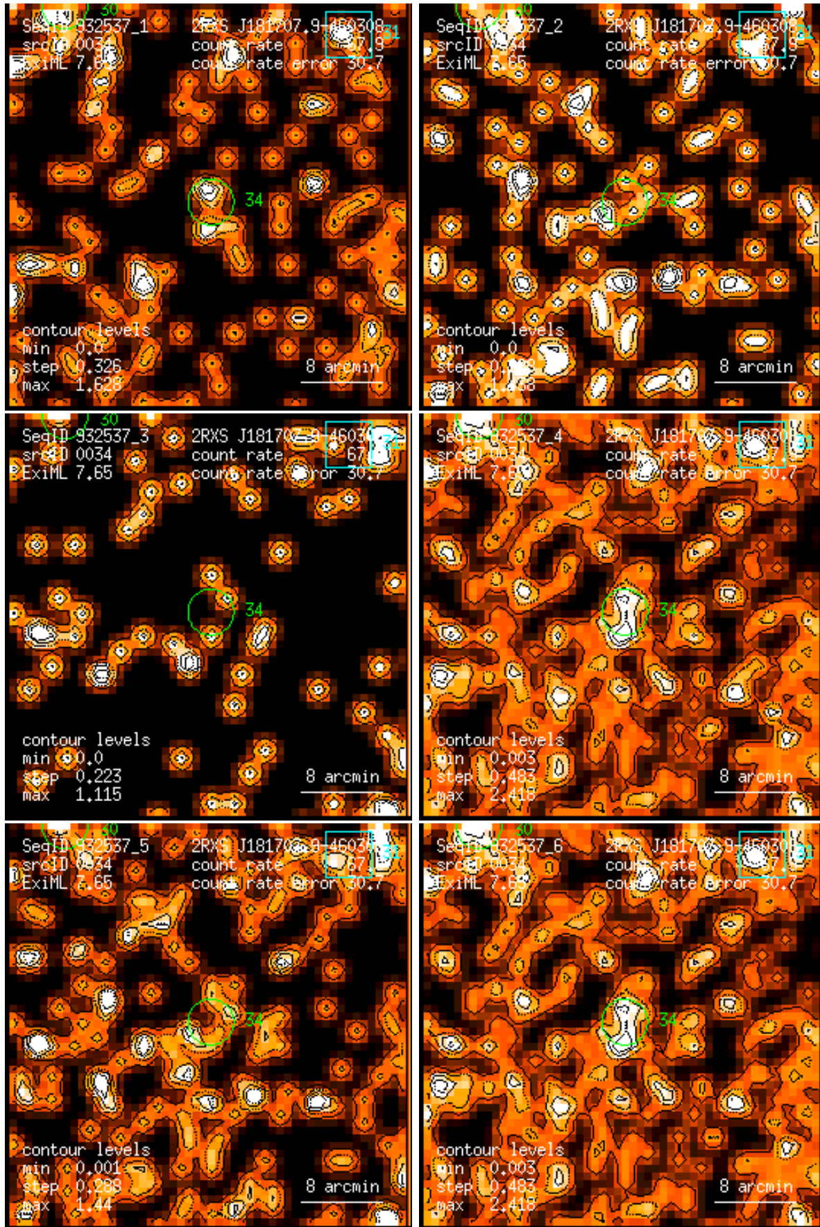
Figure 34: RASS 932537: detection 0034: band rate images, Gaussian filter: (1) PSPC channels 11 – 41, (2) 52 – 90, (3) 91 – 201, (4) 11 – 235, (5) 52 – 201, (6) 11 – 201. Broad band rates in counts/ks. Band rate contour levels in counts/ks/arcmin 2 .
