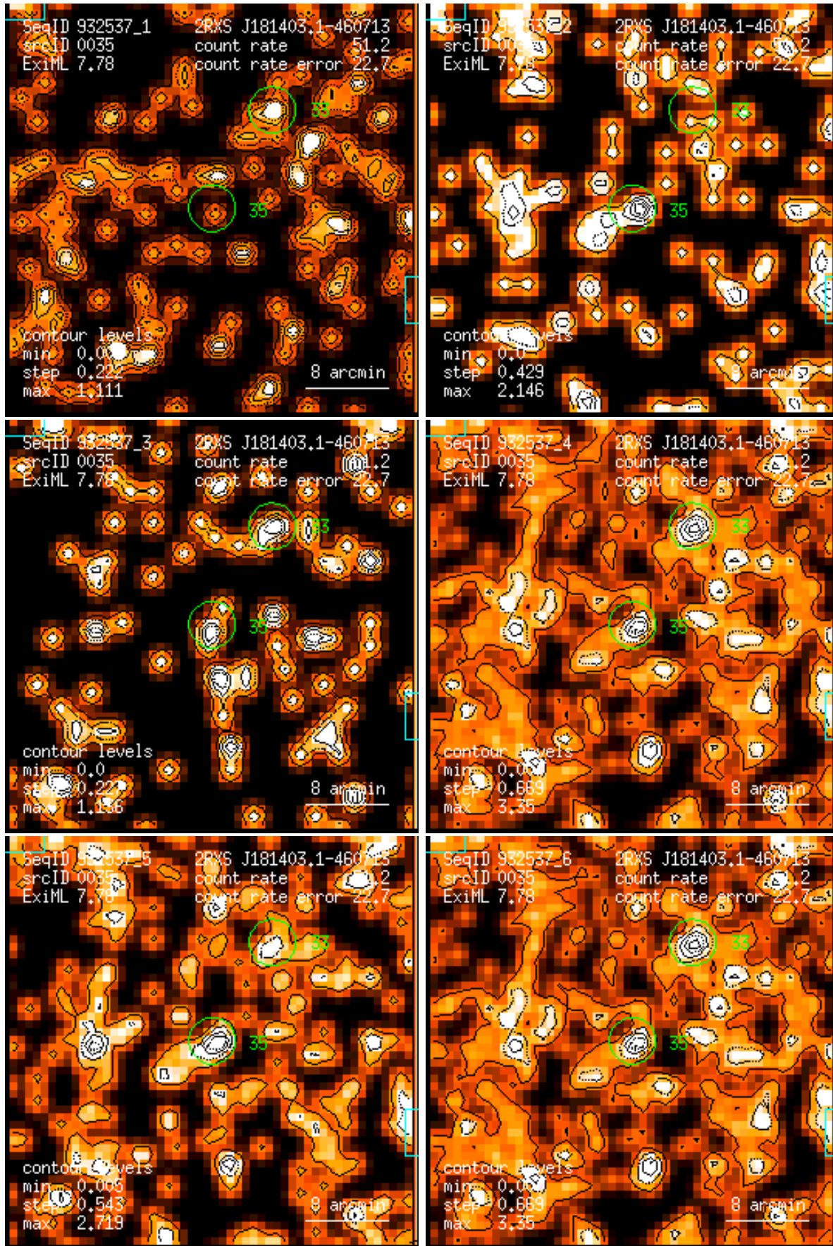
Figure 35: RASS 932537: detection 0035: band rate images, Gaussian filter: (1) PSPC channels 11 – 41, (2) 52 – 90, (3) 91 – 201, (4) 11 – 235, (5) 52 – 201, (6) 11 – 201. Broad band rates in counts/ks. Band rate contour levels in counts/ks/arcmin 2 .
