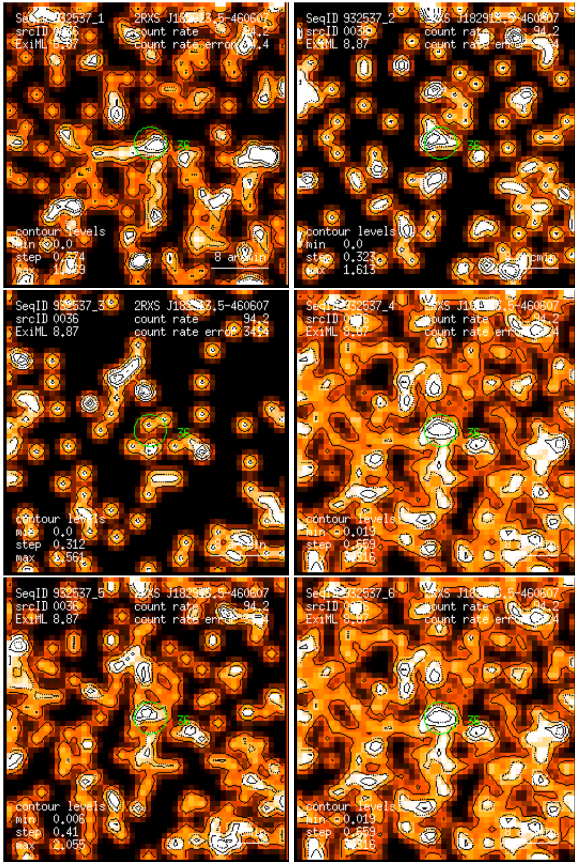
Figure 36: RASS 932537: detection 0036: band rate images, Gaussian filter: (1) PSPC channels 11 – 41, (2) 52 – 90, (3) 91 – 201, (4) 11 – 235, (5) 52 – 201, (6) 11 – 201. Broad band rates in counts/ks. Band rate contour levels in counts/ks/arcmin 2 .
