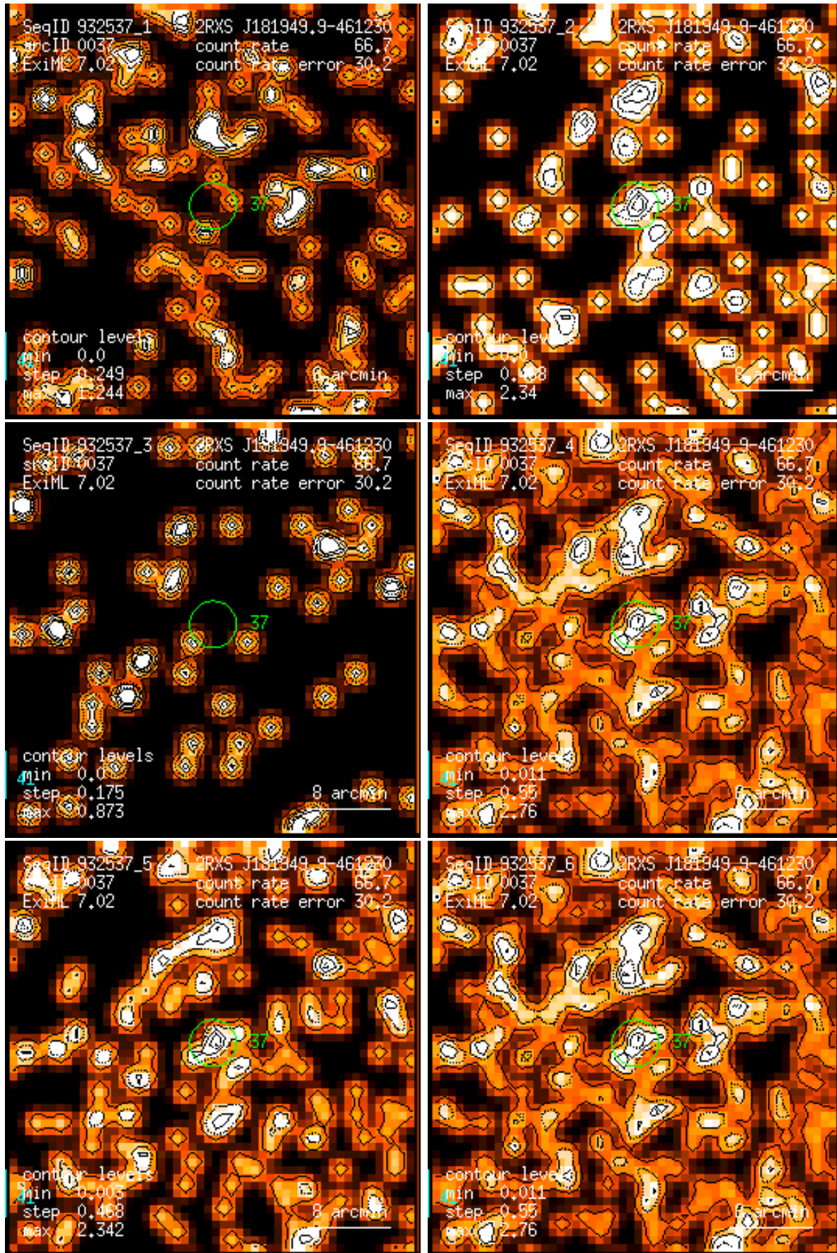
Figure 37: RASS 932537: detection 0037: band rate images, Gaussian filter: (1) PSPC channels 11 – 41, (2) 52 – 90, (3) 91 – 201, (4) 11 – 235, (5) 52 – 201, (6) 11 – 201. Broad band rates in counts/ks. Band rate contour levels in counts/ks/arcmin 2 .
