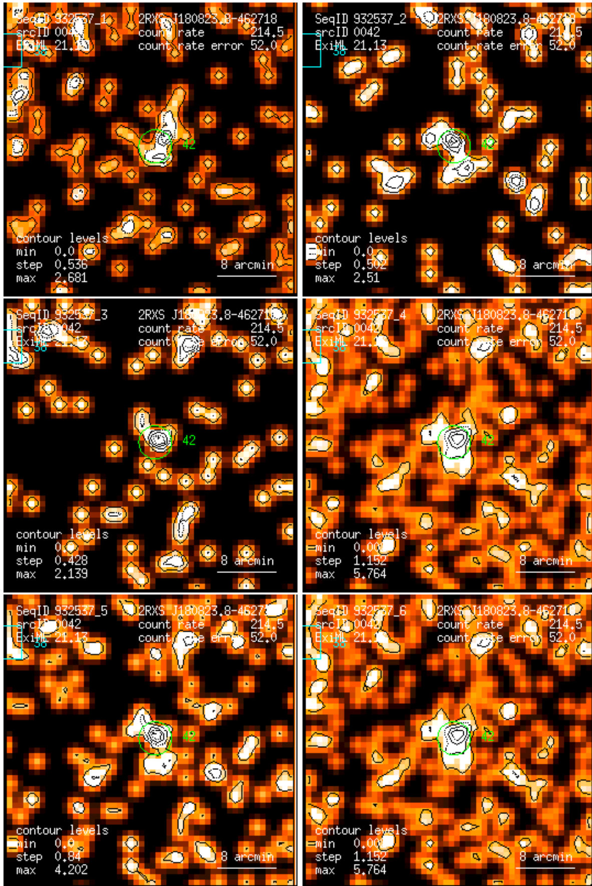
Figure 42: RASS 932537: detection 0042: band rate images, Gaussian filter: (1) PSPC channels 11 – 41, (2) 52 – 90, (3) 91 – 201, (4) 11 – 235, (5) 52 – 201, (6) 11 – 201. Broad band rates in counts/ks. Band rate contour levels in counts/ks/arcmin 2 .
