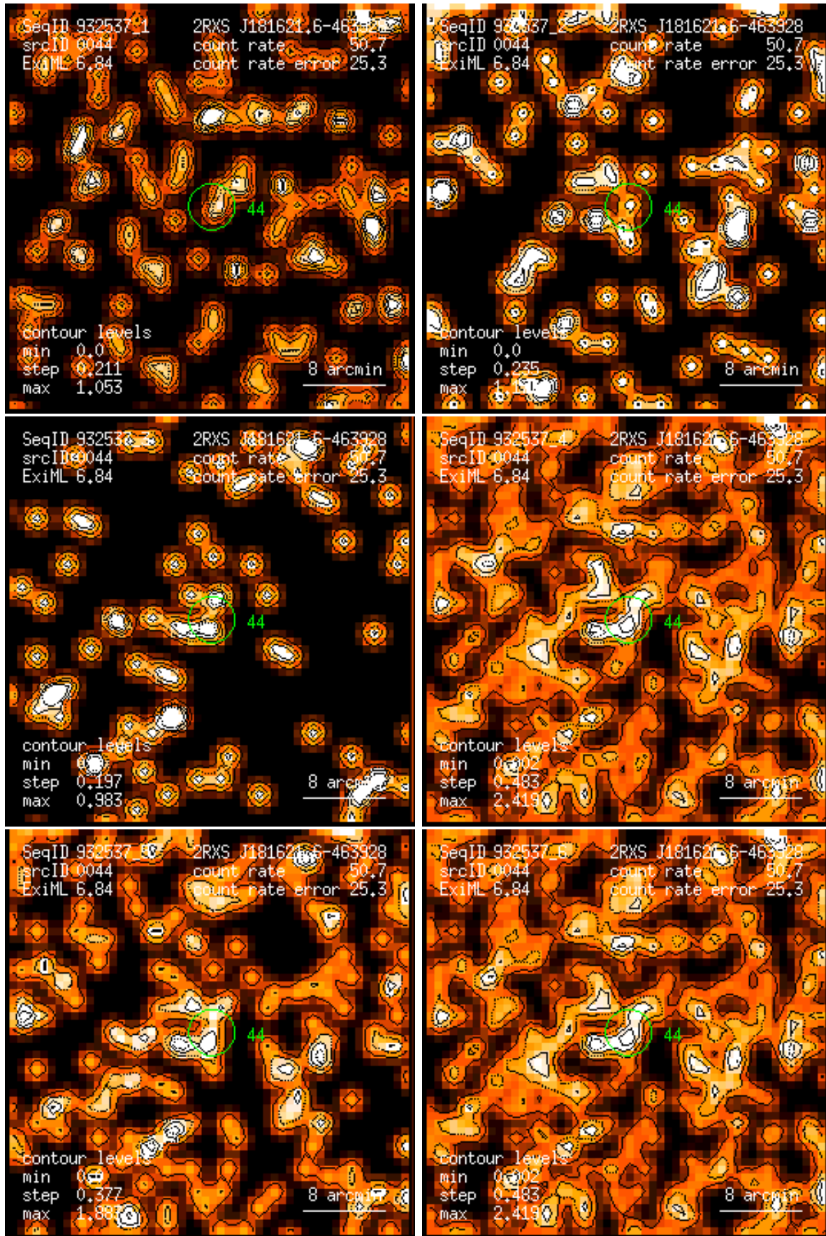
Figure 44: RASS 932537: detection 0044: band rate images, Gaussian filter: (1) PSPC channels 11 – 41, (2) 52 – 90, (3) 91 – 201, (4) 11 – 235, (5) 52 – 201, (6) 11 – 201. Broad band rates in counts/ks. Band rate contour levels in counts/ks/arcmin 2 .
