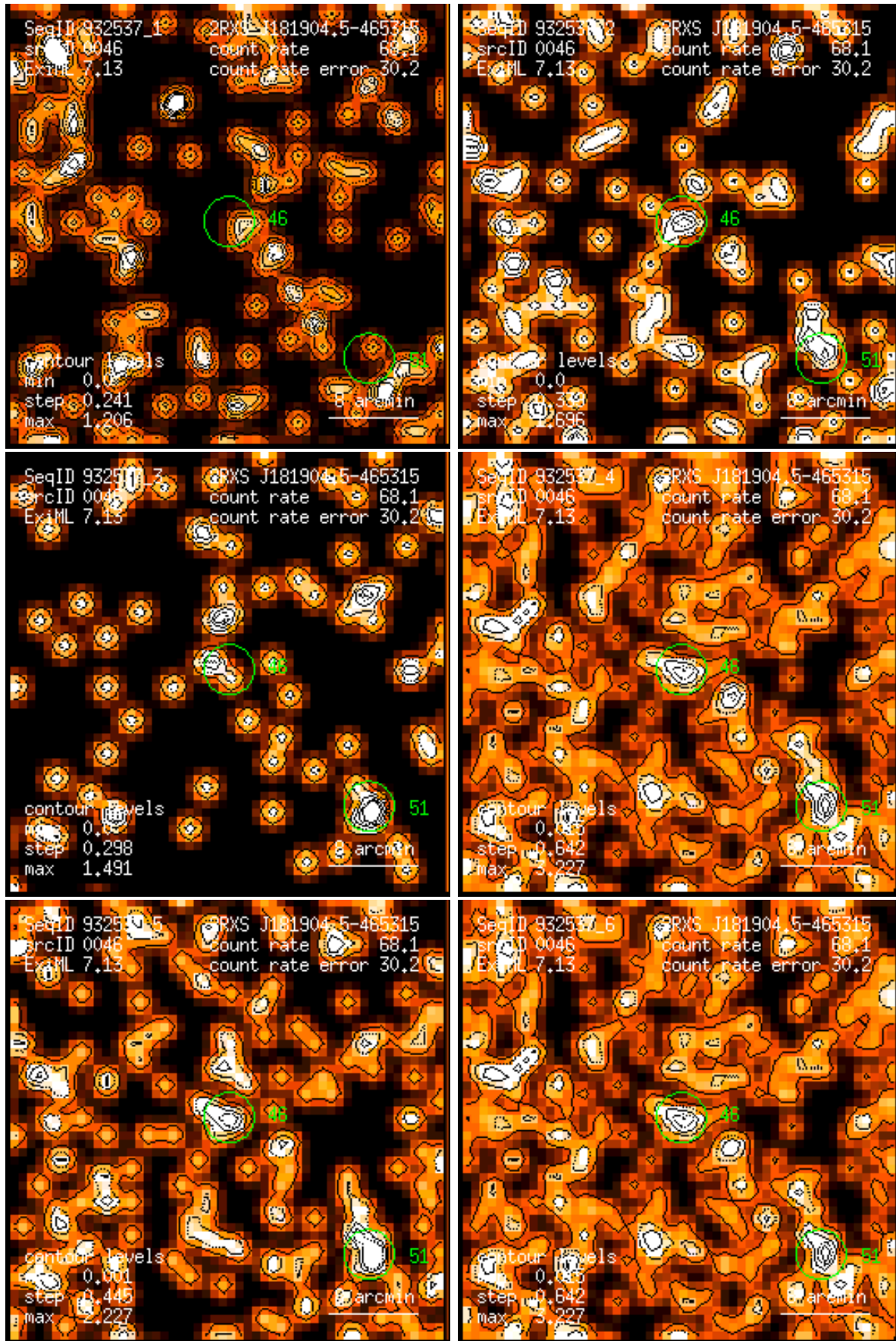
Figure 46: RASS 932537: detection 0046: band rate images, Gaussian filter: (1) PSPC channels 11 – 41, (2) 52 – 90, (3) 91 – 201, (4) 11 – 235, (5) 52 – 201, (6) 11 – 201. Broad band rates in counts/ks. Band rate contour levels in counts/ks/arcmin 2 .
