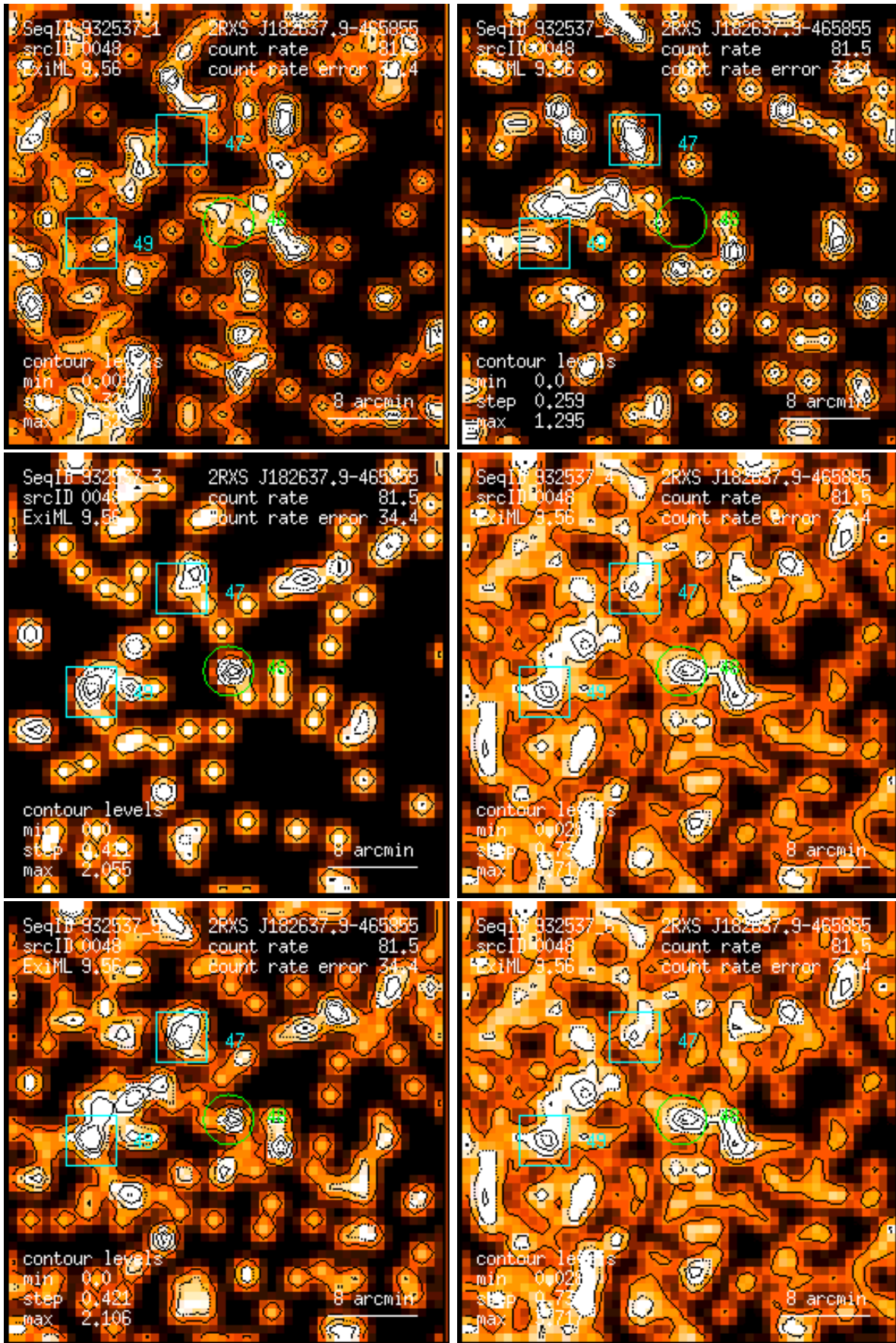
Figure 48: RASS 932537: detection 0048: band rate images, Gaussian filter: (1) PSPC channels 11 – 41, (2) 52 – 90, (3) 91 – 201, (4) 11 – 235, (5) 52 – 201, (6) 11 – 201. Broad band rates in counts/ks. Band rate contour levels in counts/ks/arcmin 2 .
