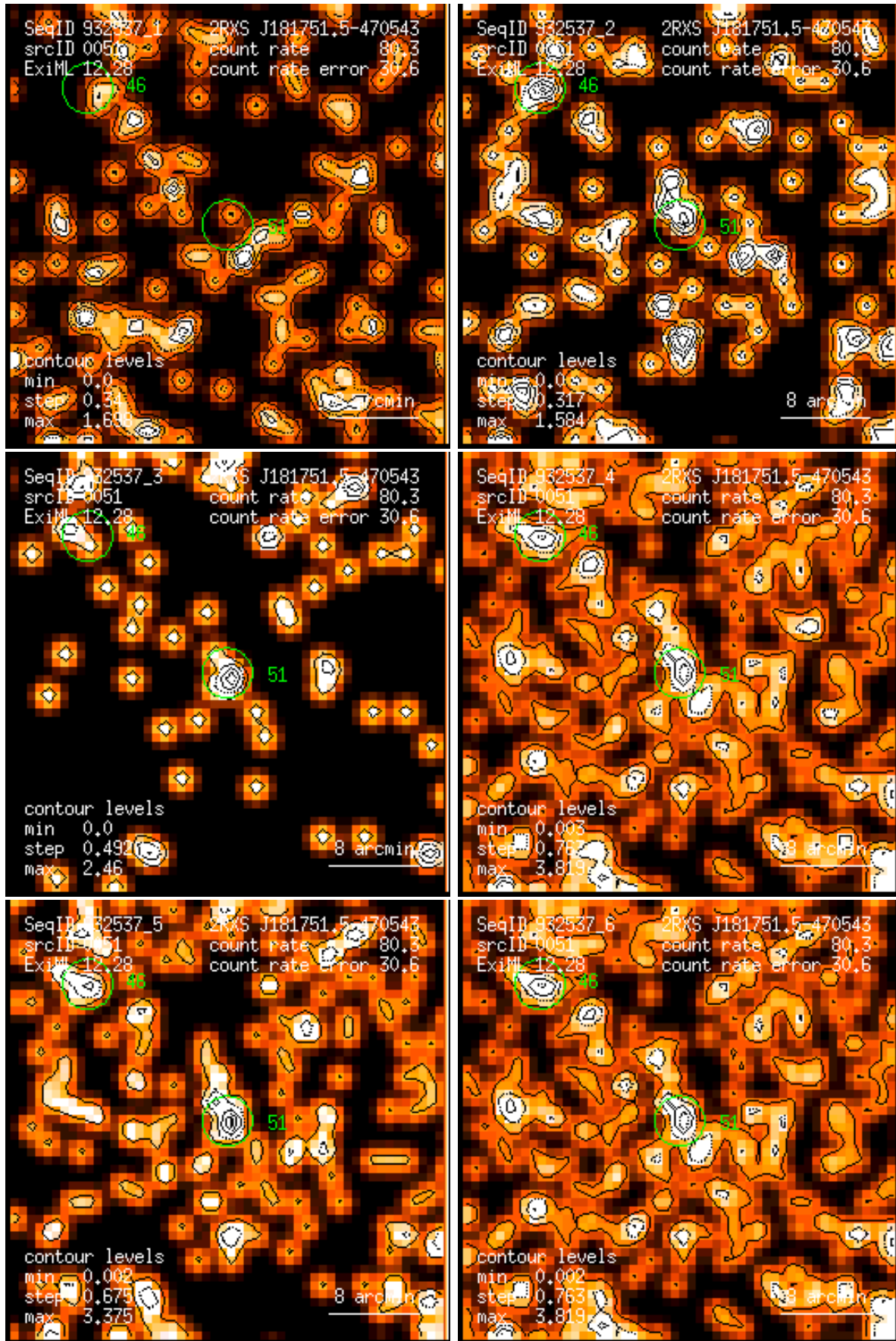
Figure 51: RASS 932537: detection 0051: band rate images, Gaussian filter: (1) PSPC channels 11 – 41, (2) 52 – 90, (3) 91 – 201, (4) 11 – 235, (5) 52 – 201, (6) 11 – 201. Broad band rates in counts/ks. Band rate contour levels in counts/ks/arcmin 2 .
