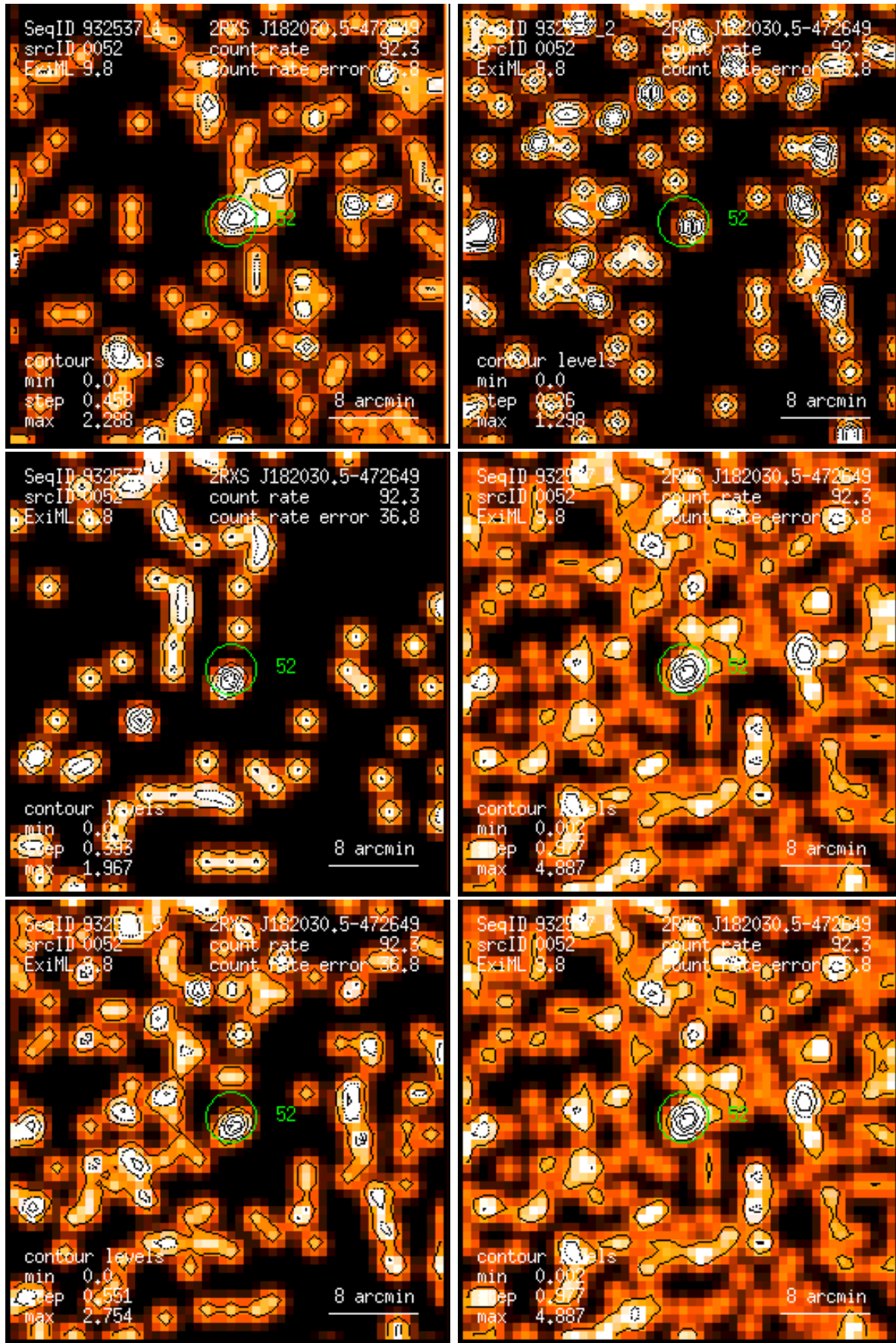
Figure 52: RASS 932537: detection 0052: band rate images, Gaussian filter: (1) PSPC channels 11 – 41, (2) 52 – 90, (3) 91 – 201, (4) 11 – 235, (5) 52 – 201, (6) 11 – 201. Broad band rates in counts/ks. Band rate contour levels in counts/ks/arcmin 2 .
