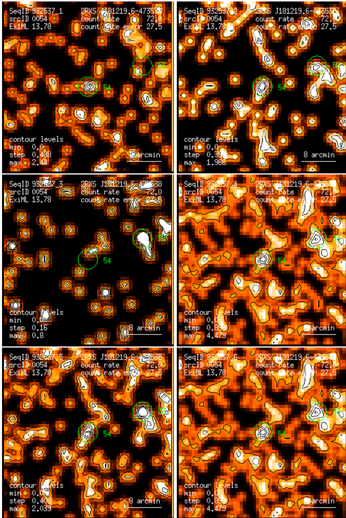
Figure 54: RASS 932537: detection 0054: band rate images, Gaussian filter: (1) PSPC channels 11 – 41, (2) 52 – 90, (3) 91 – 201, (4) 11 – 235, (5) 52 – 201, (6) 11 – 201. Broad band rates in counts/ks. Band rate contour levels in counts/ks/arcmin 2 .
