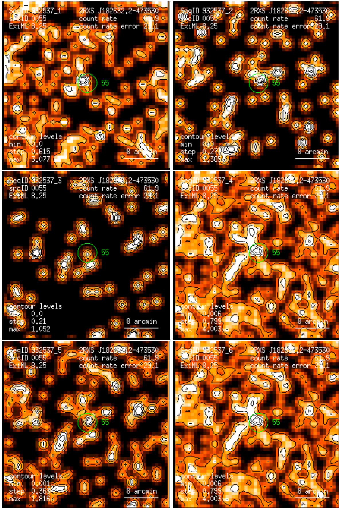
Figure 55: RASS 932537: detection 0055: band rate images, Gaussian filter: (1) PSPC channels 11 – 41, (2) 52 – 90, (3) 91 – 201, (4) 11 – 235, (5) 52 – 201, (6) 11 – 201. Broad band rates in counts/ks. Band rate contour levels in counts/ks/arcmin 2 .
