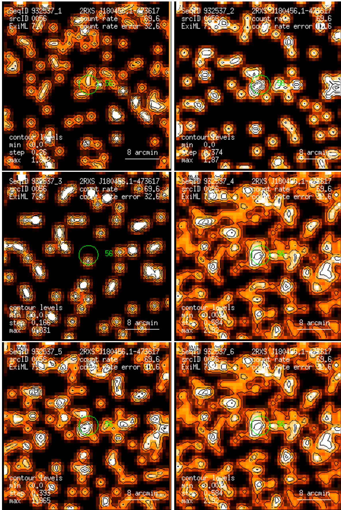
Figure 56: RASS 932537: detection 0056: band rate images, Gaussian filter: (1) PSPC channels 11 – 41, (2) 52 – 90, (3) 91 – 201, (4) 11 – 235, (5) 52 – 201, (6) 11 – 201. Broad band rates in counts/ks. Band rate contour levels in counts/ks/arcmin 2 .
