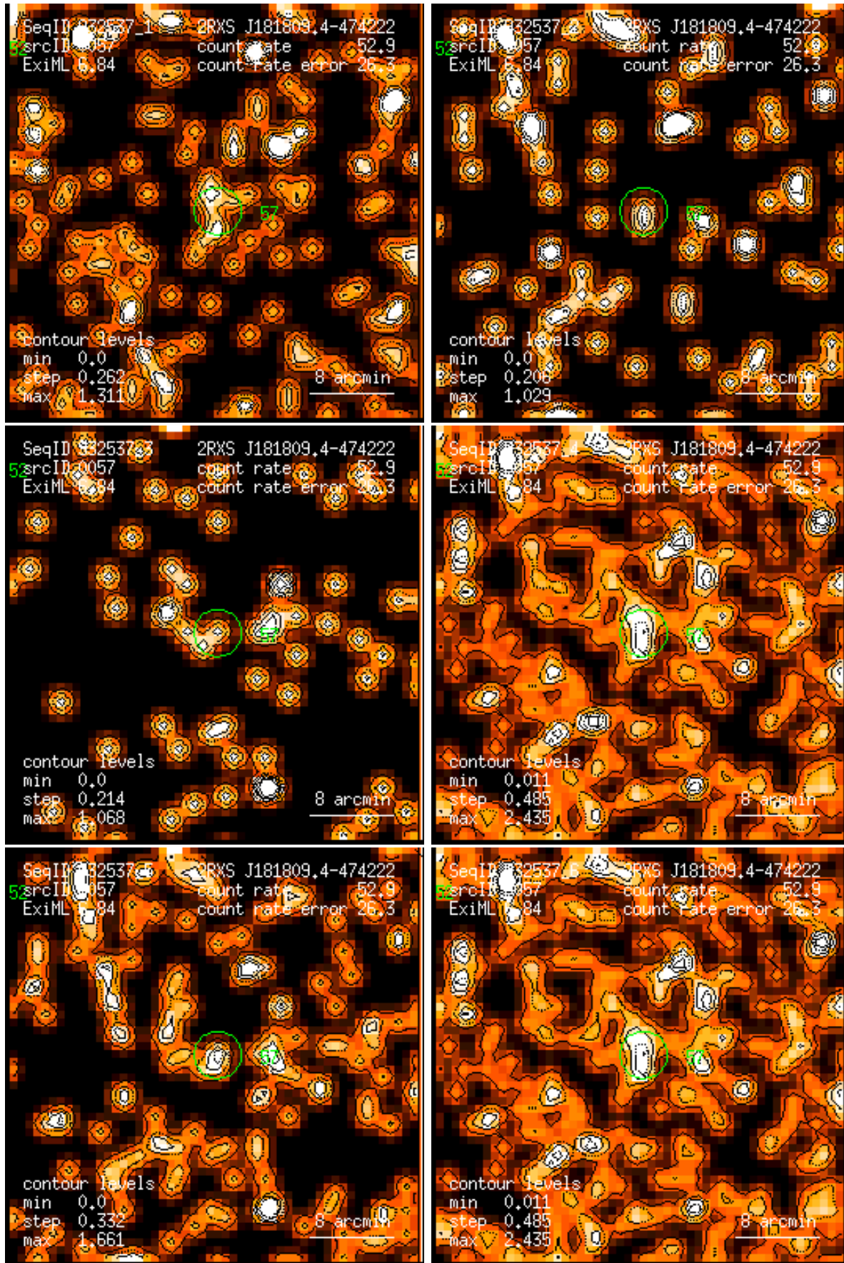
Figure 57: RASS 932537: detection 0057: band rate images, Gaussian filter: (1) PSPC channels 11 – 41, (2) 52 – 90, (3) 91 – 201, (4) 11 – 235, (5) 52 – 201, (6) 11 – 201. Broad band rates in counts/ks. Band rate contour levels in counts/ks/arcmin 2 .
