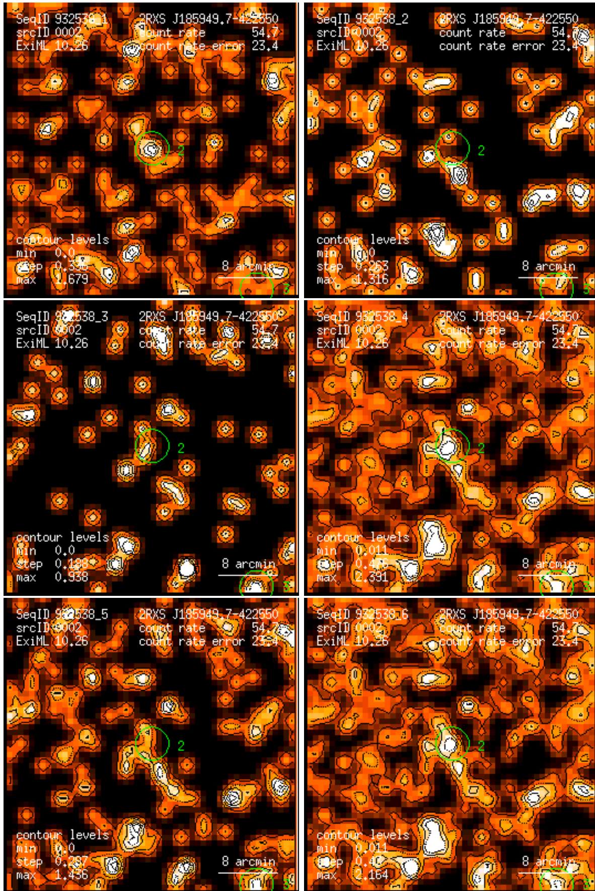
Figure 2: RASS 932538: detection 0002: band rate images, Gaussian filter: (1) PSPC channels 11 – 41, (2) 52 – 90, (3) 91 – 201, (4) 11 – 235, (5) 52 – 201, (6) 11 – 201. Broad band rates in counts/ks. Band rate contour levels in counts/ks/arcmin 2 .
