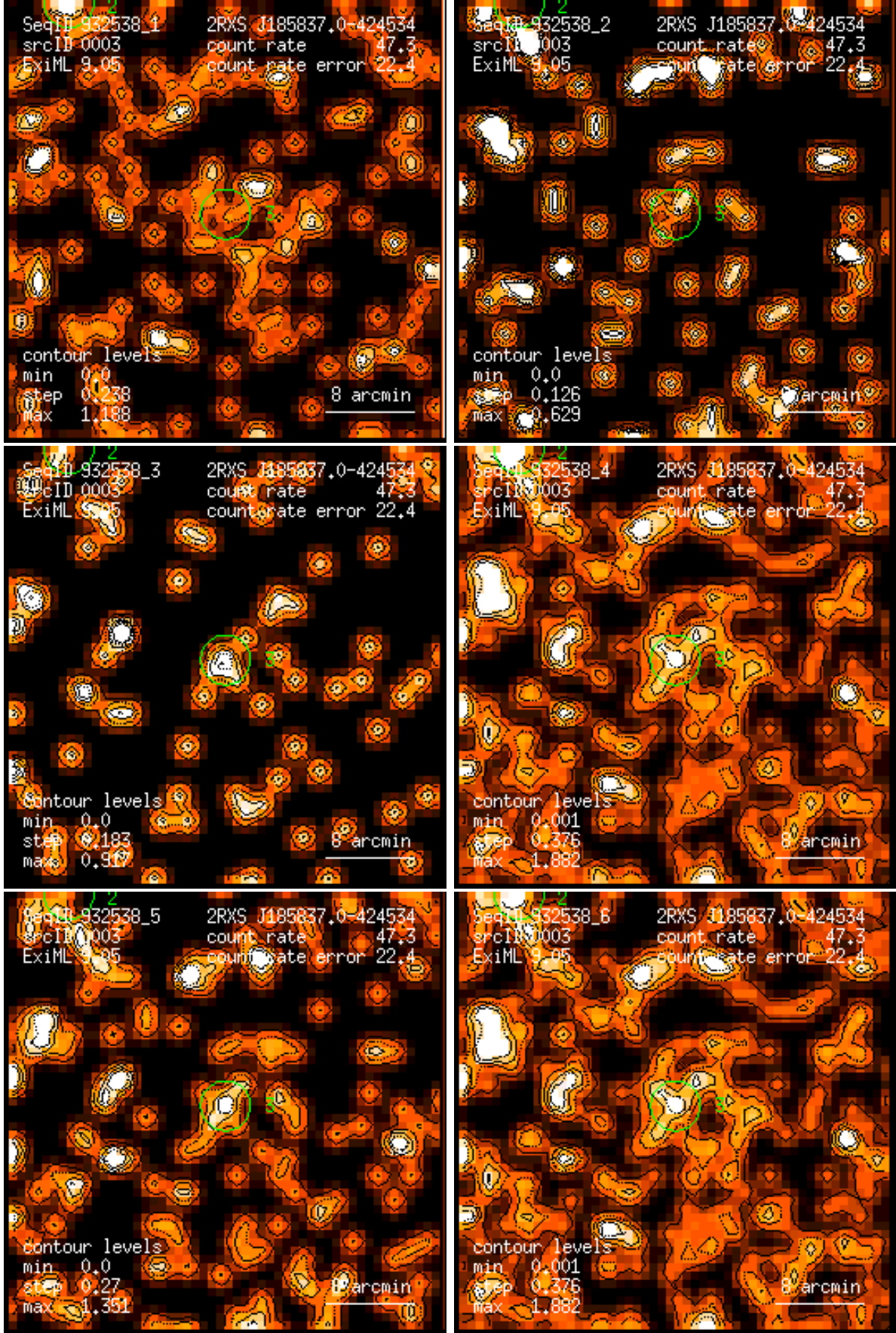
Figure 3: RASS 932538: detection 0003: band rate images, Gaussian filter: (1) PSPC channels 11 – 41, (2) 52 – 90, (3) 91 – 201, (4) 11 – 235, (5) 52 – 201, (6) 11 – 201. Broad band rates in counts/ks. Band rate contour levels in counts/ks/arcmin 2 .
