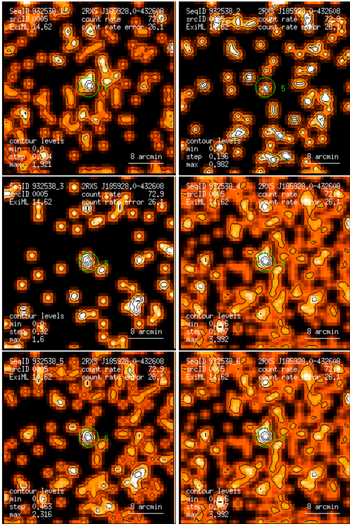
Figure 5: RASS 932538: detection 0005: band rate images, Gaussian filter: (1) PSPC channels 11 – 41, (2) 52 – 90, (3) 91 – 201, (4) 11 – 235, (5) 52 – 201, (6) 11 – 201. Broad band rates in counts/ks. Band rate contour levels in counts/ks/arcmin 2 .
