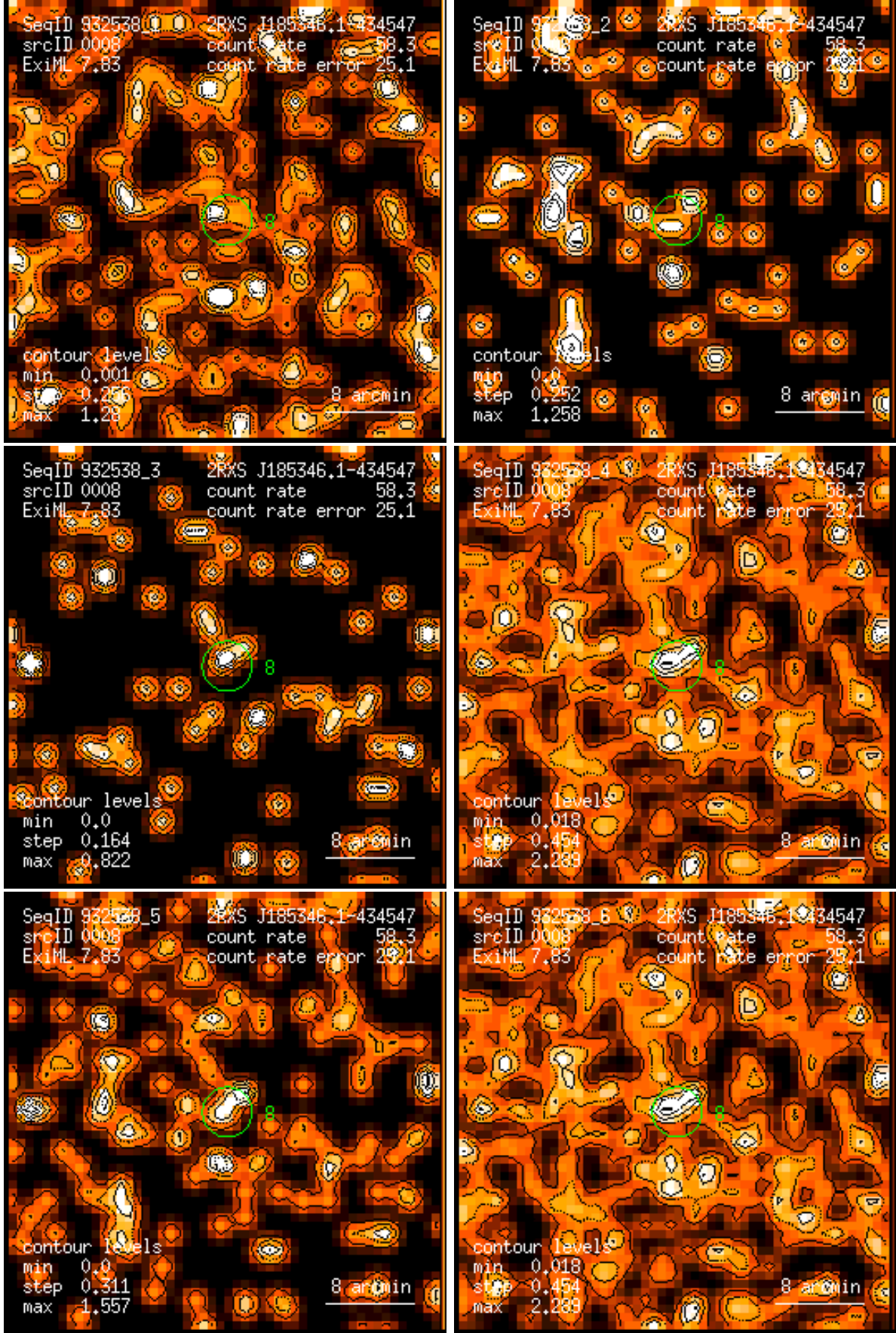
Figure 8: RASS 932538: detection 0008: band rate images, Gaussian filter: (1) PSPC channels 11 – 41, (2) 52 – 90, (3) 91 – 201, (4) 11 – 235, (5) 52 – 201, (6) 11 – 201. Broad band rates in counts/ks. Band rate contour levels in counts/ks/arcmin 2 .
