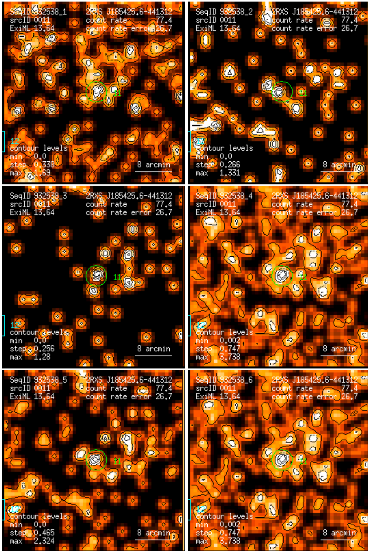
Figure 11: RASS 932538: detection 0011: band rate images, Gaussian filter: (1) PSPC channels 11 – 41, (2) 52 – 90, (3) 91 – 201, (4) 11 – 235, (5) 52 – 201, (6) 11 – 201. Broad band rates in counts/ks. Band rate contour levels in counts/ks/arcmin 2 .
