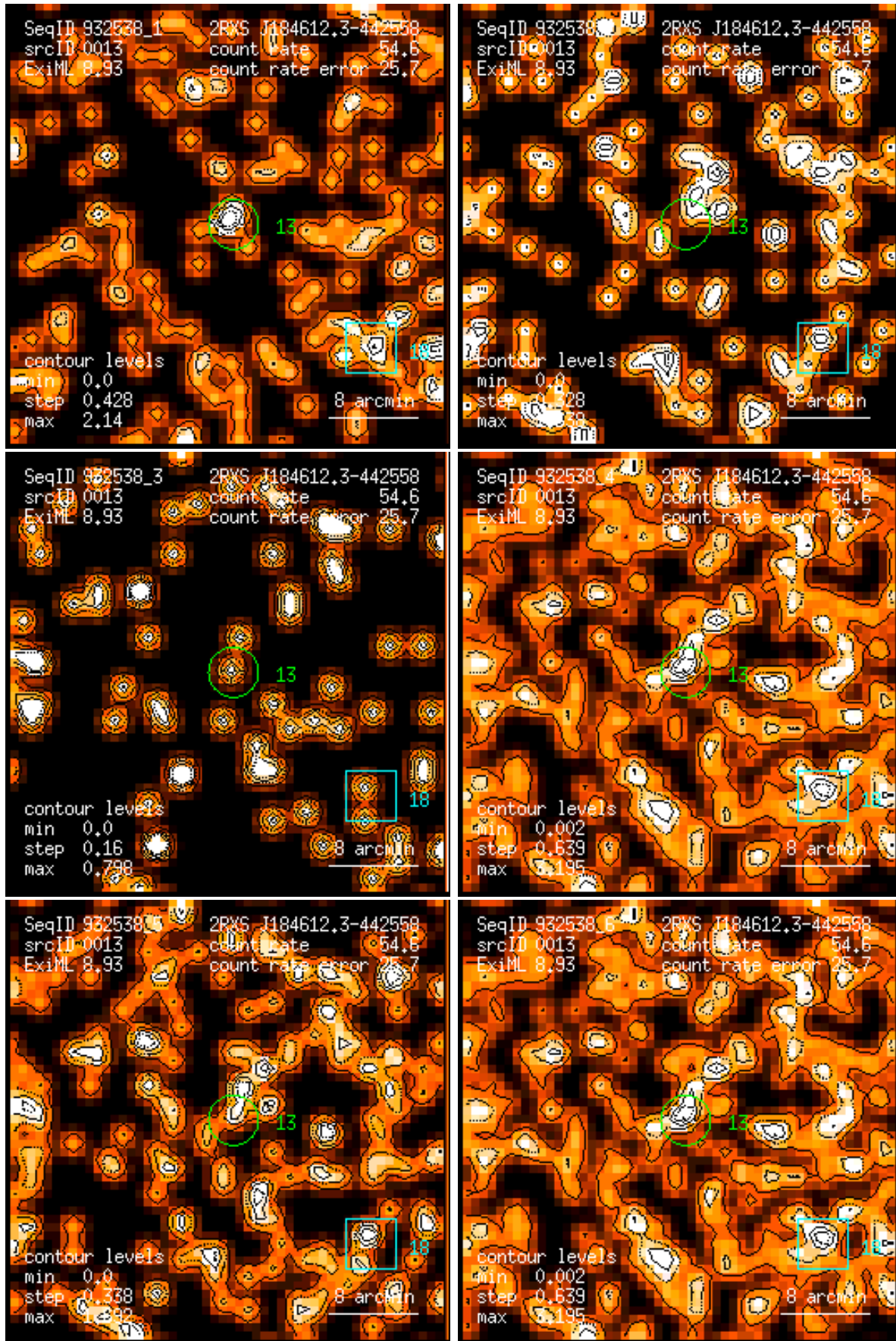
Figure 13: RASS 932538: detection 0013: band rate images, Gaussian filter: (1) PSPC channels 11 – 41, (2) 52 – 90, (3) 91 – 201, (4) 11 – 235, (5) 52 – 201, (6) 11 – 201. Broad band rates in counts/ks. Band rate contour levels in counts/ks/arcmin 2 .
